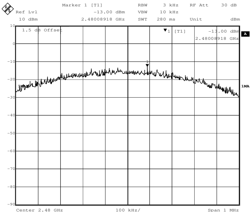
Channel 39:2.480 GHz:
