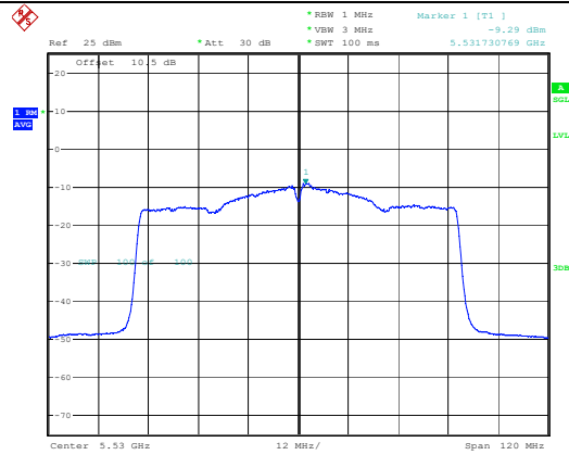
Maximum power spectral density
