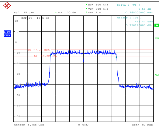
6dB Emission Bandwidth
