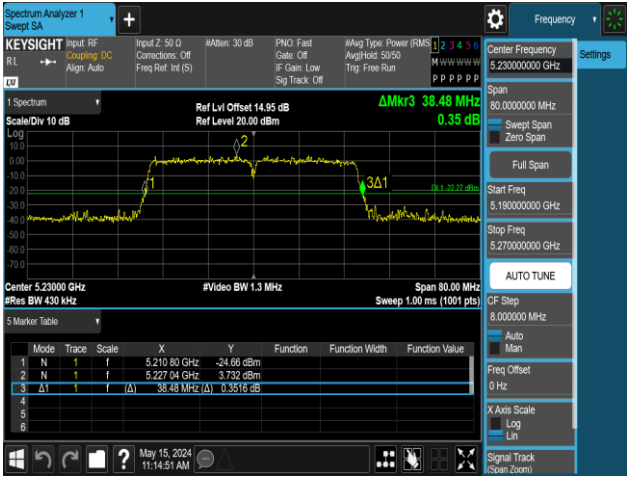
11AC40MIMO-Ant2-5230
