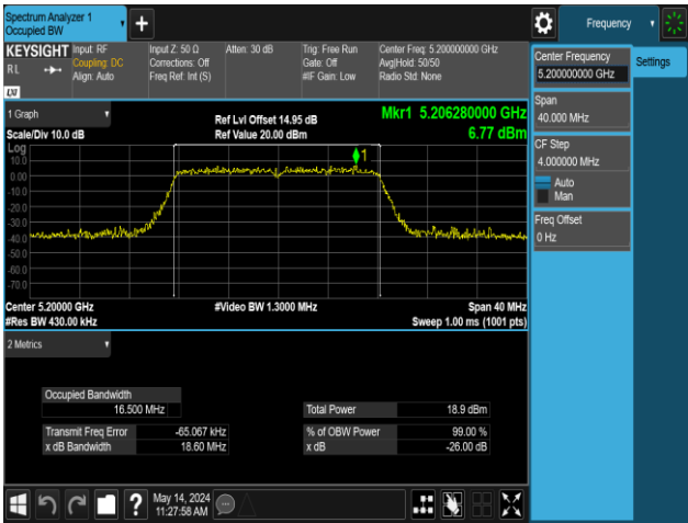
11A-Ant2-5200
