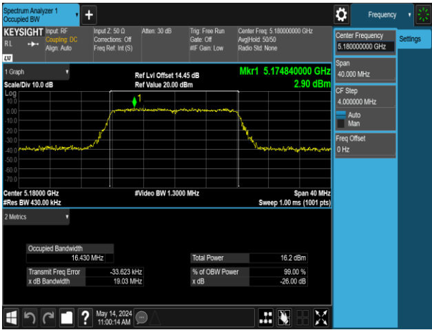
11A-Ant1-5180
