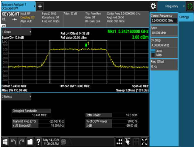
11A-Ant1-5240
