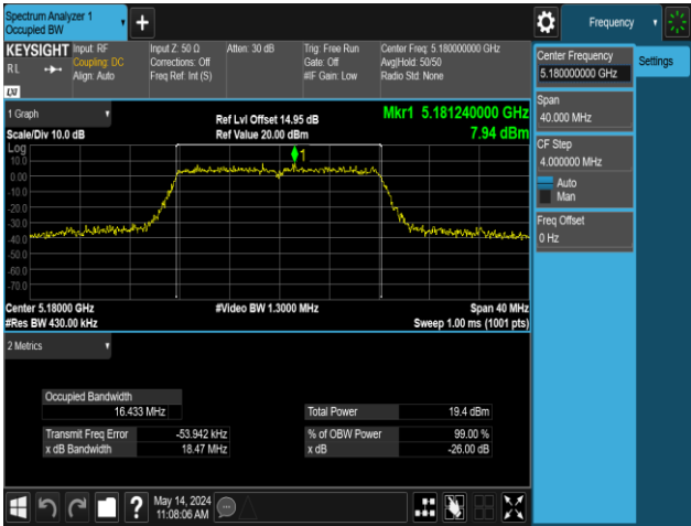
11A-Ant2-5180
