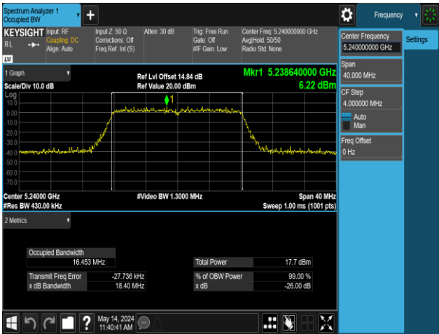
11A-Ant2-5240
