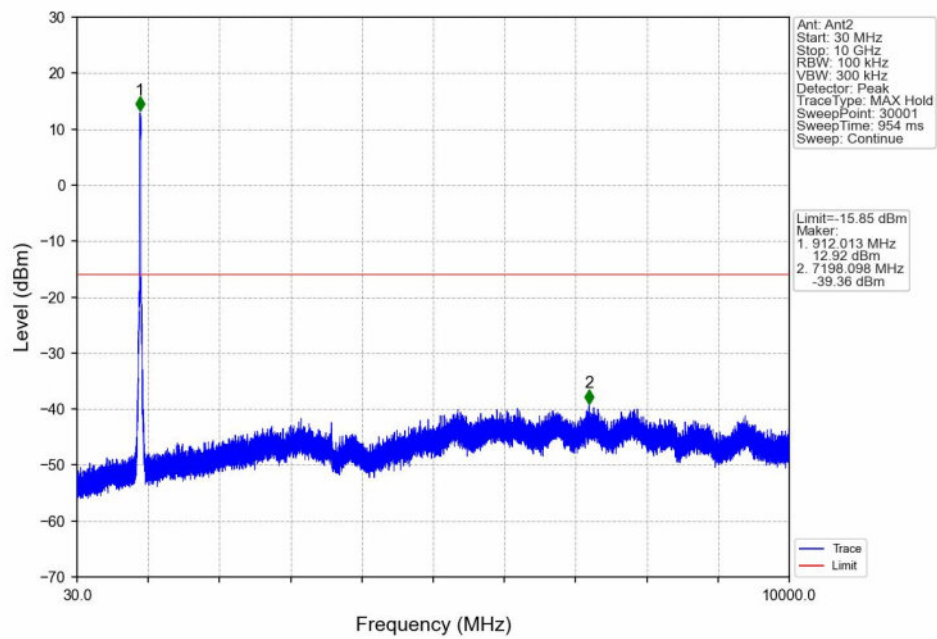
QPSK_LCH_914MHz_Ant2_NTNV
