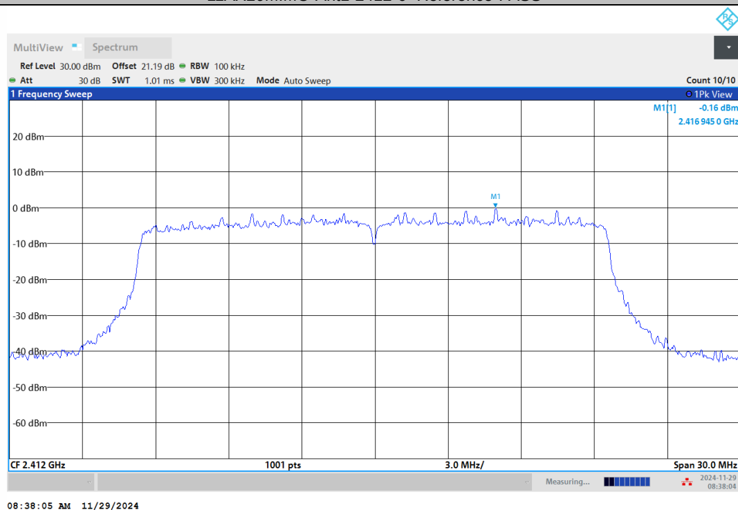
11AX20MIMO-Ant2-2412-0~Reference-PASS
