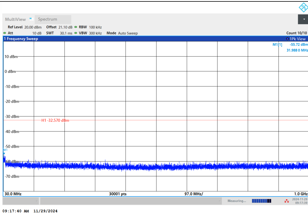
11AX40MIMO-Ant1-2422-30~1000-PASS
