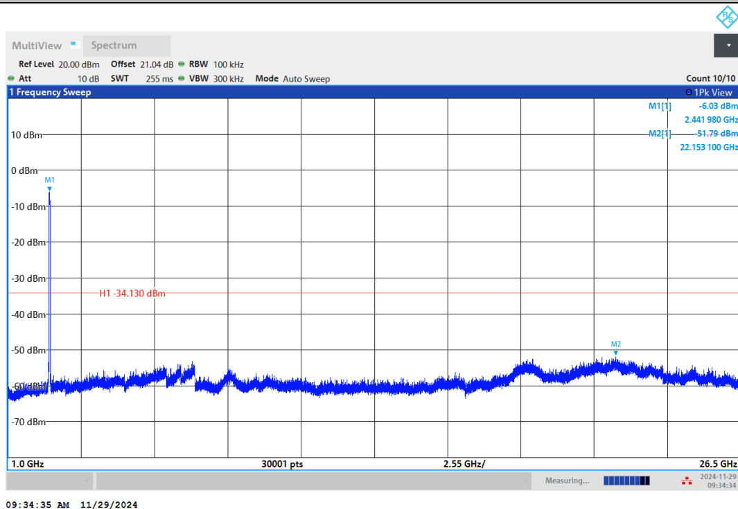
11AX40MIMO-Ant2-2437-1000~26500-PASS
