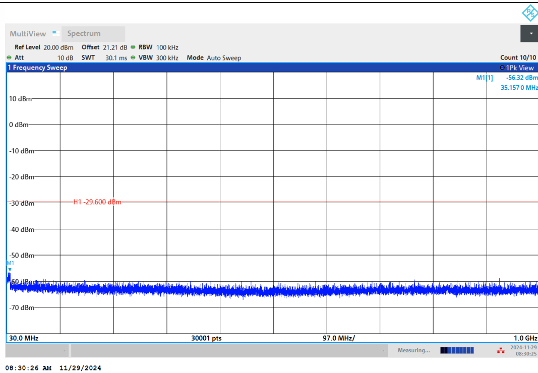
11AX20MIMO-Ant1-2412-30~1000-PASS
