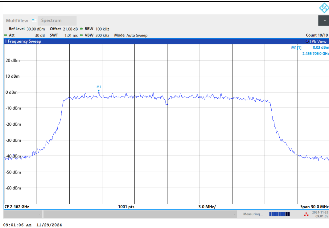
11AX20MIMO-Ant1-2462-0~Reference-PASS
