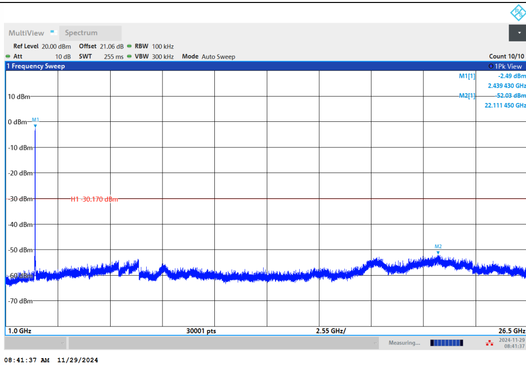
11AX20MIMO-Ant1-2437-1000~26500-PASS
