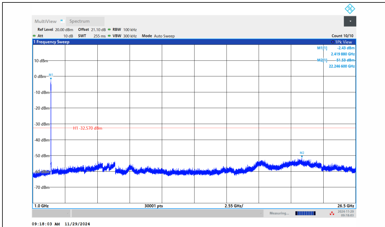
11AX40MIMO-Ant1-2422-1000~26500-PASS
