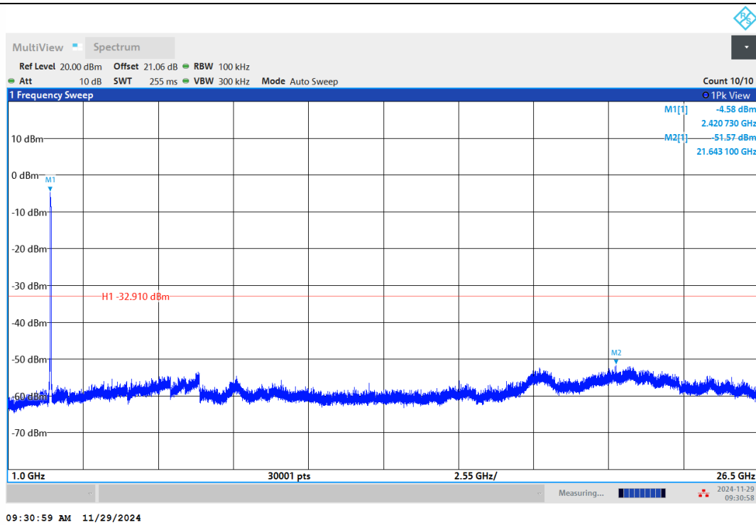
11AX40MIMO-Ant1-2437-1000~26500-PASS
