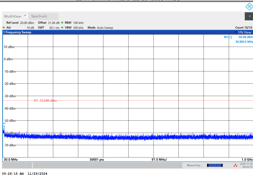
11AX40MIMO-Ant2-2422-30~1000-PASS
