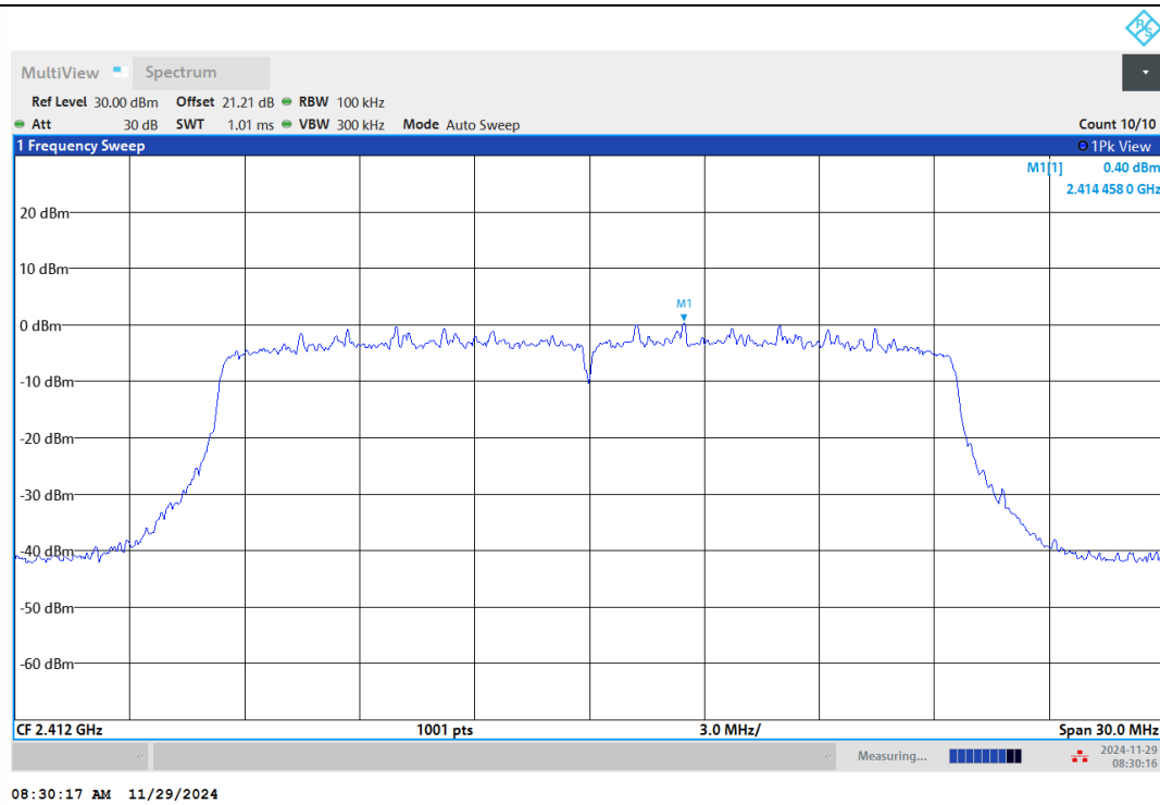
11AX20MIMO-Ant1-2412-0~Reference-PASS
