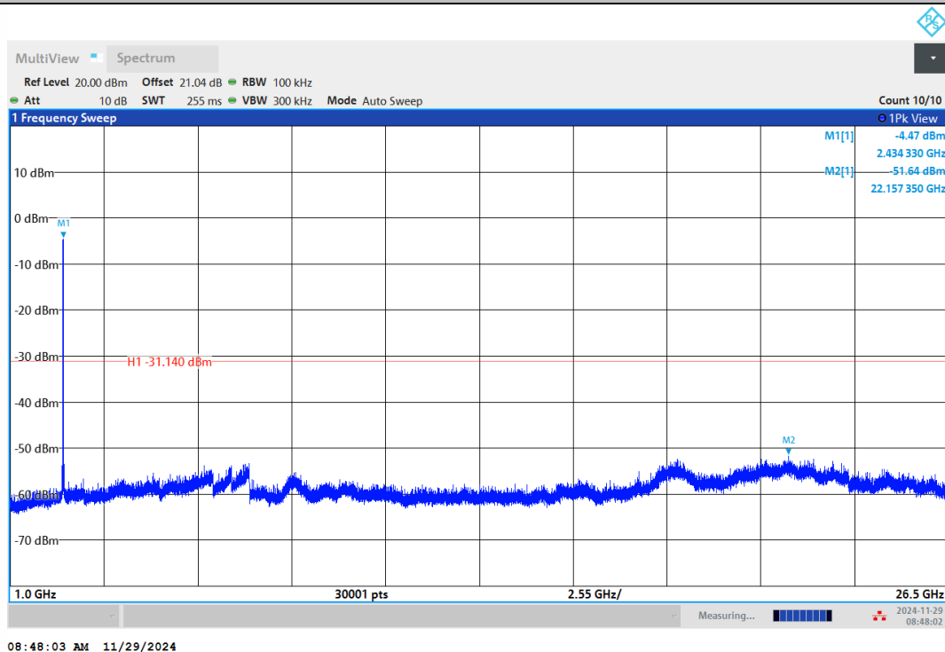
11AX20MIMO-Ant2-2437-1000~26500-PASS
