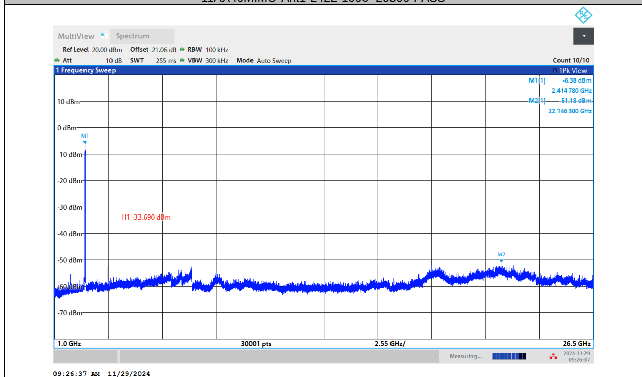
11AX40MIMO-Ant2-2422-1000~26500-PASS
