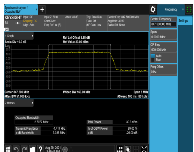
Band5-3MHz-16QAM-20635-15RB#0
