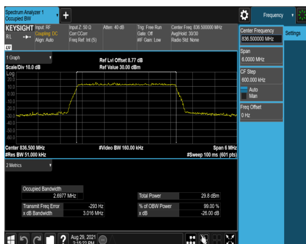
Band5-3MHz-16QAM-20525-15RB#0
