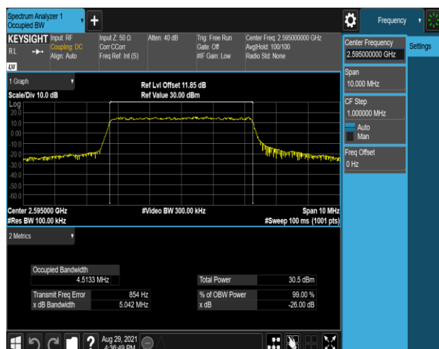
Band38-5MHz-16QAM-38000-25RB#0
