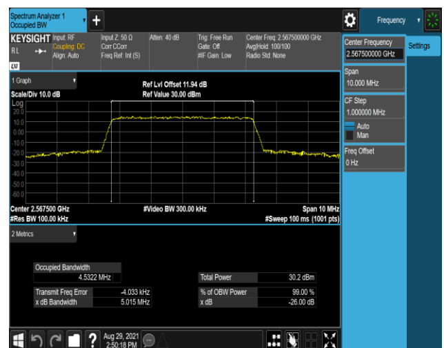
Band7-5MHz-16QAM-21425-25RB#0
