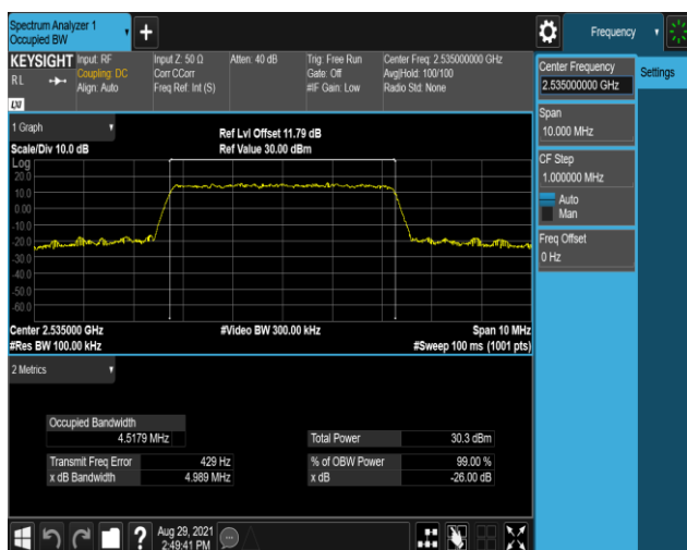
Band7-5MHz-16QAM-21100-25RB#0
