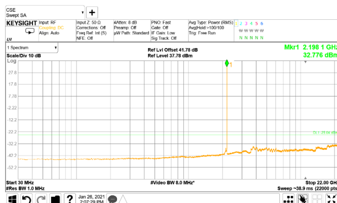
Figure 8.3-3: Conducted spurious emissions of 5 MHz top channel, single carrier operation
