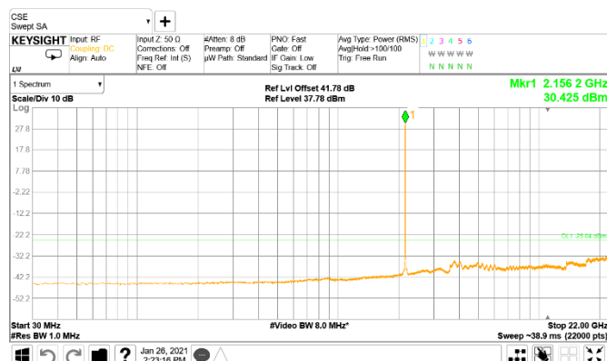
Figure 8.3-14: Conducted spurious emissions of 5 MHz two mid channels, two-carrier operation
