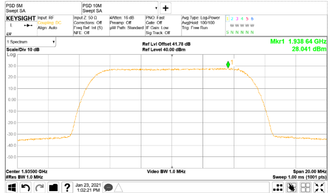
Figure 8.2-2: PSD of 10 MHz channel bandwidth, single carrier operation, sample plot
