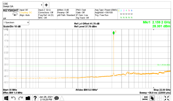
Figure 8.3-8: Conducted spurious emissions of 15 MHz mid channel, single carrier operation
