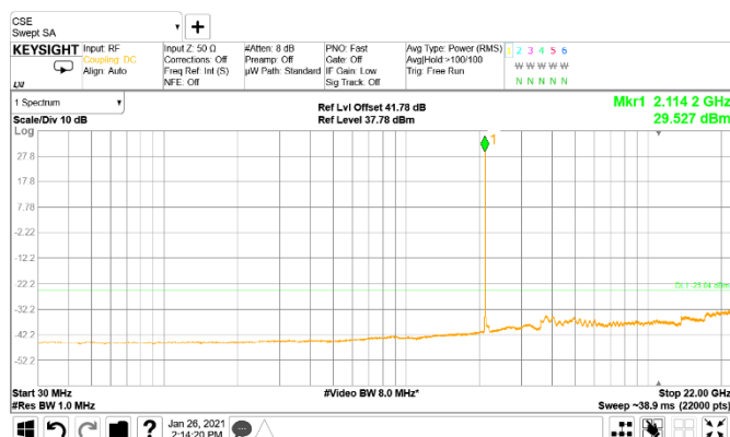
Figure 8.3-4: Conducted spurious emissions of 10 MHz low channel, single carrier operation
