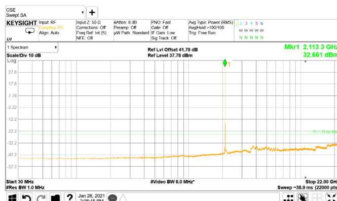
Figure 8.3-1: Conducted spurious emissions of 5 MHz low channel, single carrier operation
