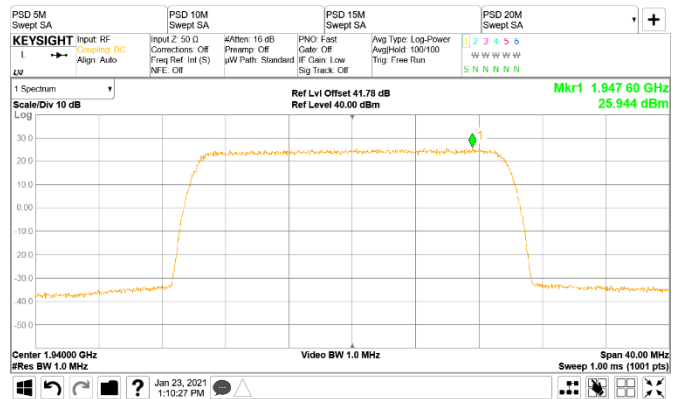
Figure 8.2-4: PSD of 20 MHz channel bandwidth, single carrier operation, sample plot
