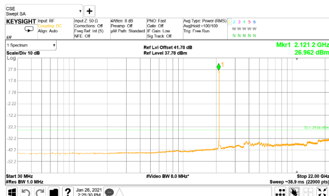
Figure 8.3-16: Conducted spurious emissions of 10 MHz two low channels, two-carrier operation
