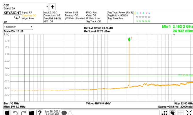
Figure 8.3-12: Conducted spurious emissions of 20 MHz top channel, single carrier operation
