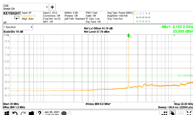
Figure 8.3-2: Conducted spurious emissions of 5 MHz mid channel, single carrier operation
