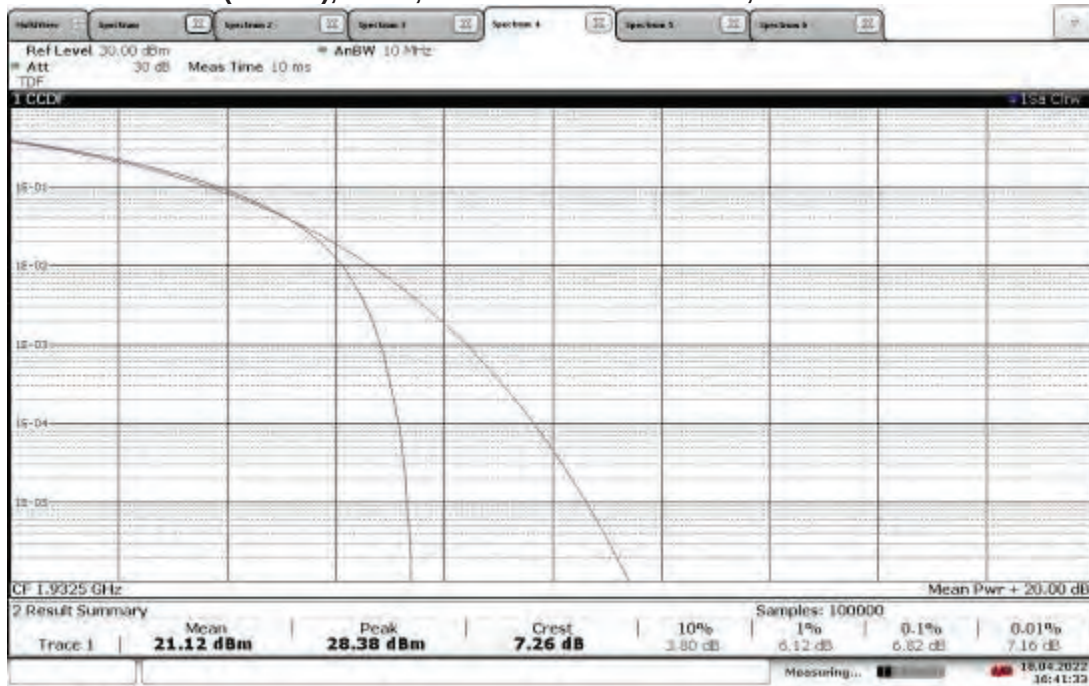
TM1.1-QPSK_5 MHz Bandwidth (4G LTE) Slot 0 (Band 2), ANT1, Low Channel 1932.5 MHz, PAPR = 7.26 dB
