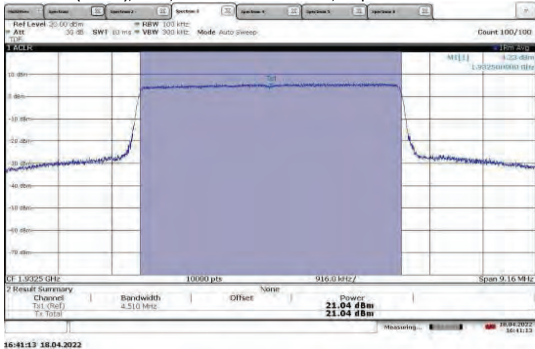
TM1.1-QPSK_5 MHz Bandwidth (4G LTE) Slot 0 (Band 2), ANT1, Low Channel 1932.5 MHz, Output Power = 21.04 dBm
