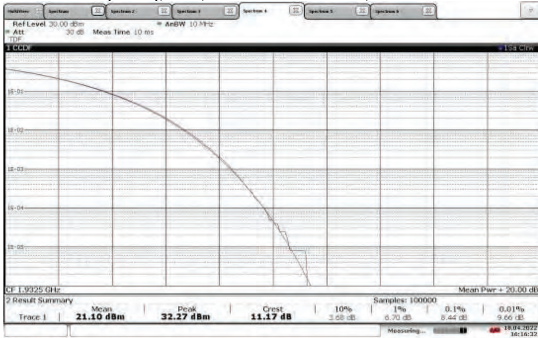
TM1.1-QPSK_5 MHz Bandwidth (4G LTE) Slot 0 (Band 2), ANT0, Low Channel 1932.5 MHz, PAPR = 11.17 dB
