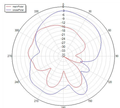
Phi=0 freq=2400MHz
