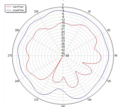
Phi=90 freq=2400MHz
