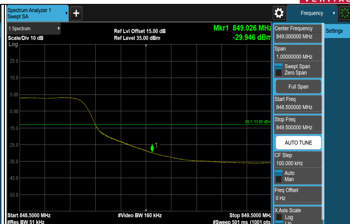
FULL CH 27015 (846.5 MHz)
