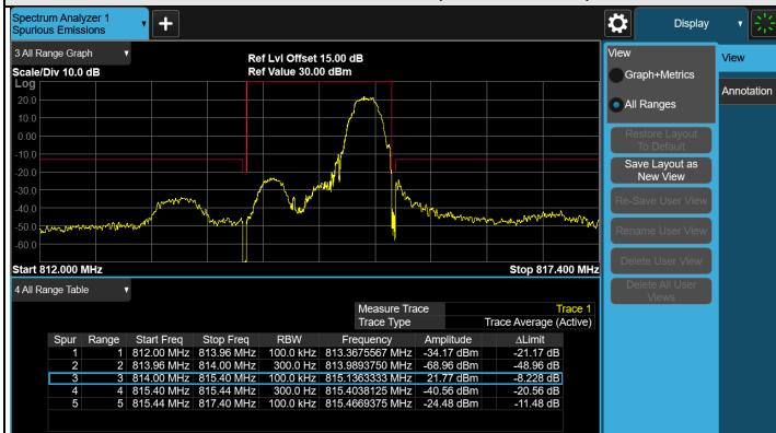
1RB#MAX CH 26697 (814.7 MHz)
