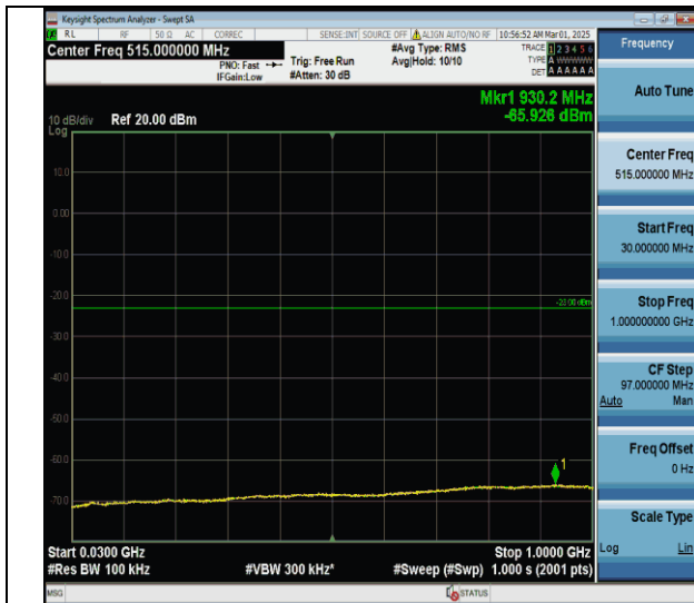
Band2-20MHz-QPSK-19100-1RB#0-30~1000-PASS
