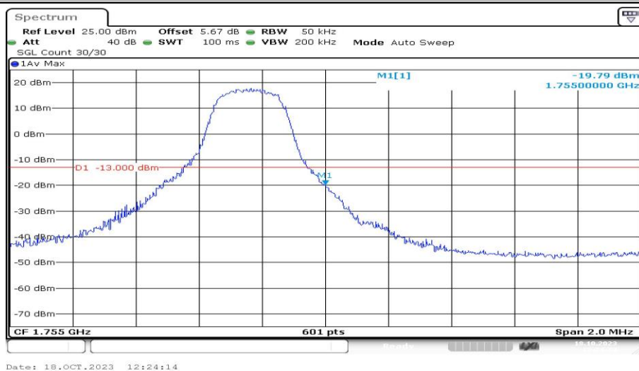
Band4-3MHz-QPSK-20385-1RB#14-PASS
