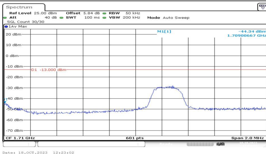
Band4-3MHz-16QAM-19965-1RB#14-PASS
