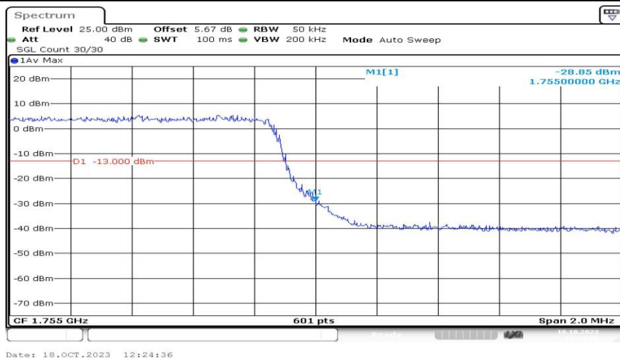
Band4-3MHz-QPSK-20385-15RB#0-PASS
