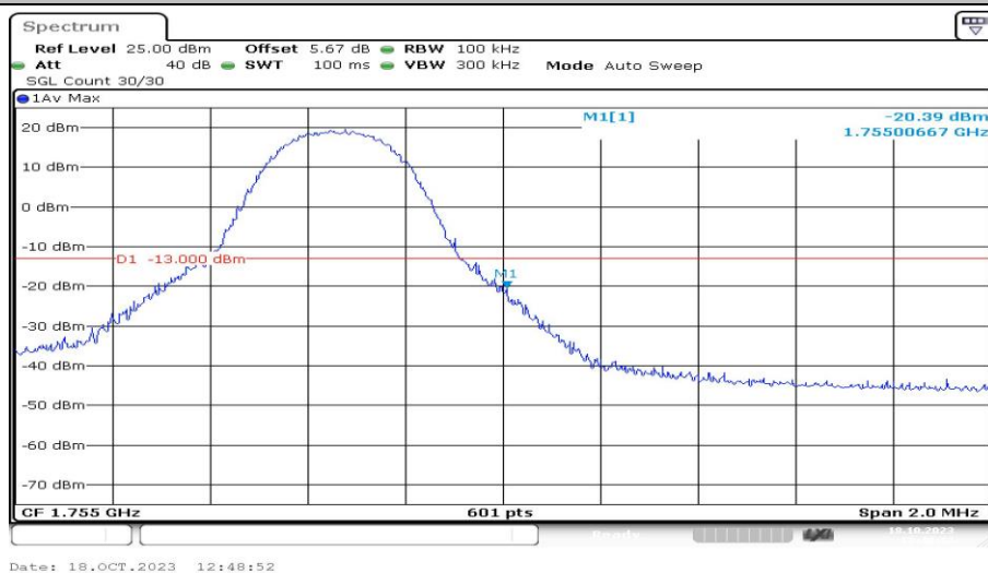
Band4-5MHz-QPSK-20375-1RB#24-PASS
