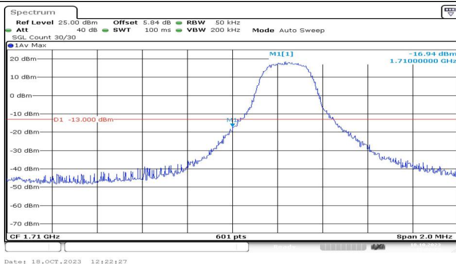
Band4-3MHz-QPSK-19965-1RB#0-PASS
