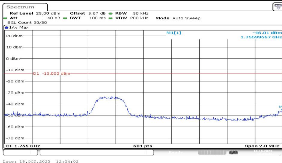
Band4-3MHz-16QAM-20385-1RB#0-PASS
