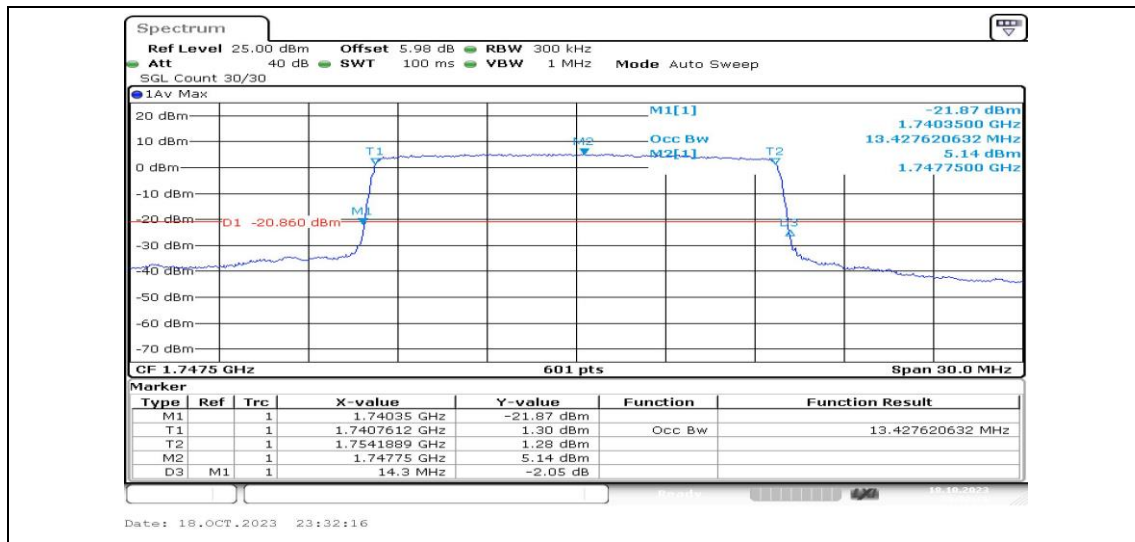
Band4-15MHz-QPSK-20325-75RB#0-PASS
