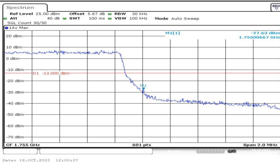
Band4-1.4MHz-16QAM-20393-6RB#0-PASS
