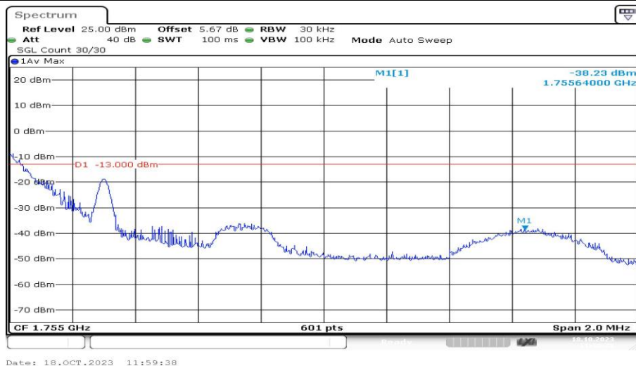
Band4-1.4MHz-QPSK-20393-1RB#0-PASS
