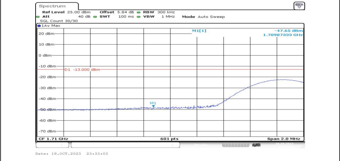
Band4-15MHz-QPSK-20025-1RB#74-PASS
