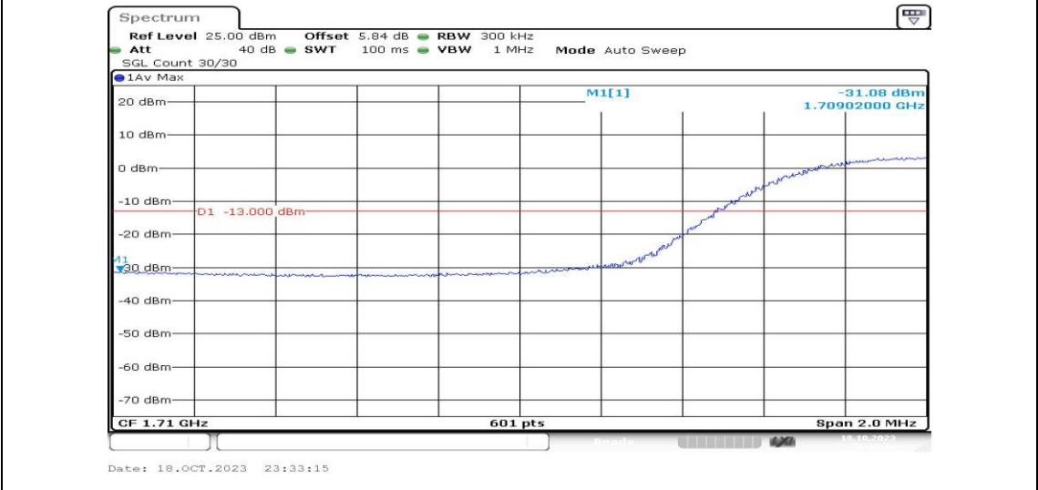
Band4-15MHz-QPSK-20025-75RB#0-PASS
