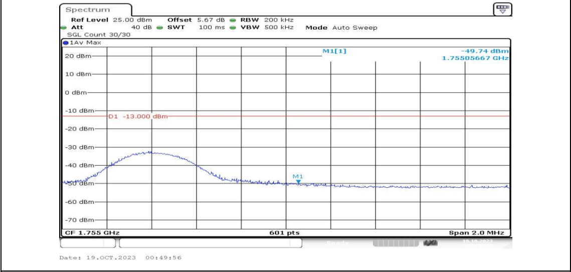
Band4-10MHz-16QAM-20350-1RB#0-PASS
