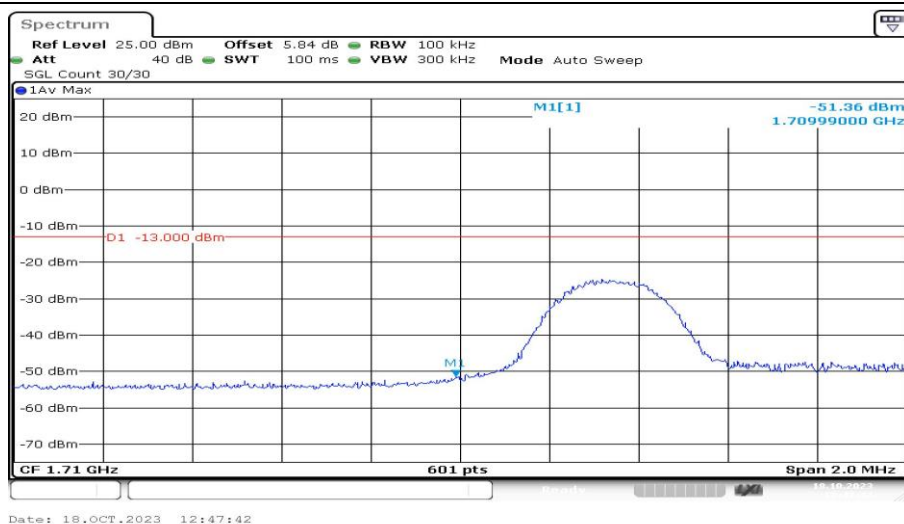
Band4-5MHz-16QAM-19975-1RB#24-PASS
