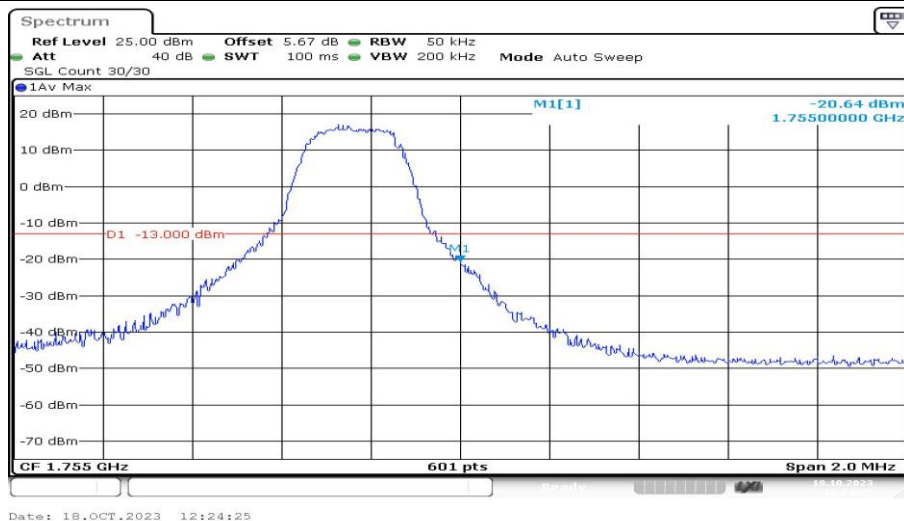
Band4-3MHz-16QAM-20385-1RB#14-PASS
