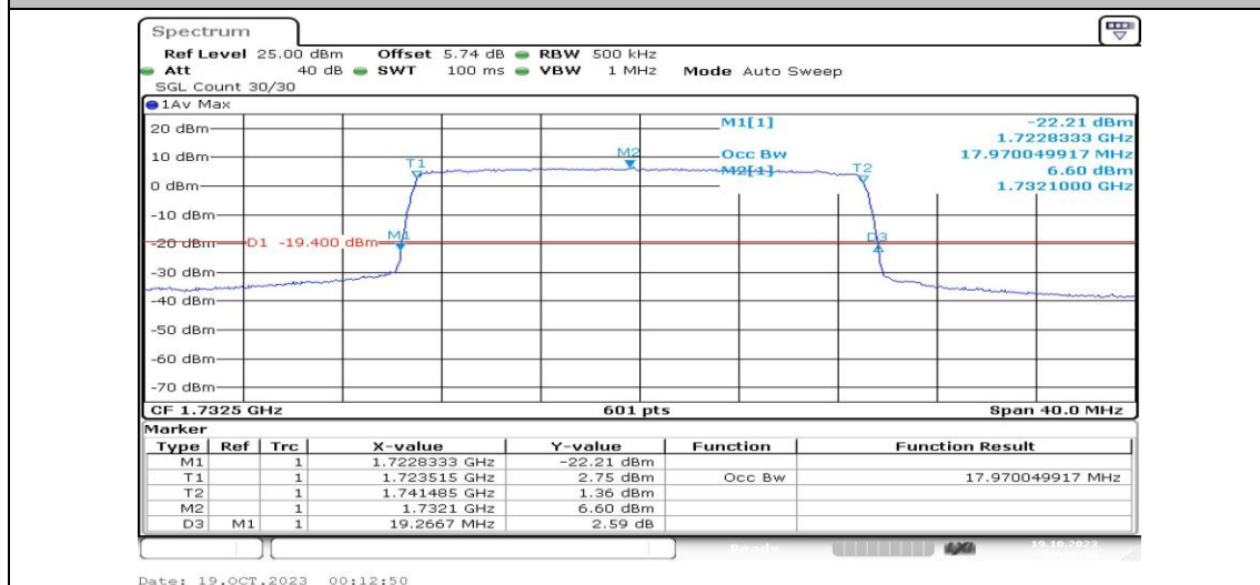
Band4-20MHz-QPSK-20175-100RB#0-PASS
