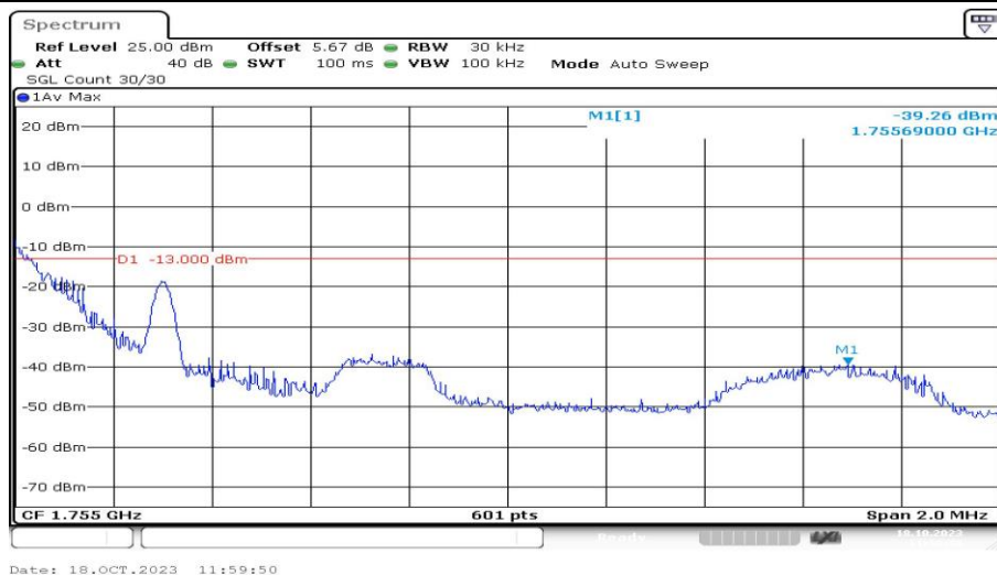
Band4-1.4MHz-16QAM-20393-1RB#0-PASS
