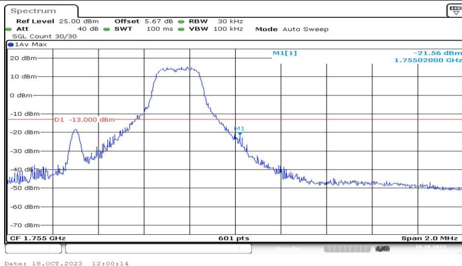
Band4-1.4MHz-16QAM-20393-1RB#5-PASS
