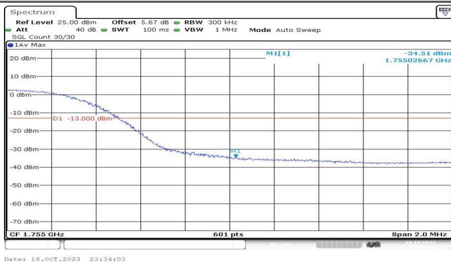
Band4-15MHz-QPSK-20325-75RB#0-PASS
