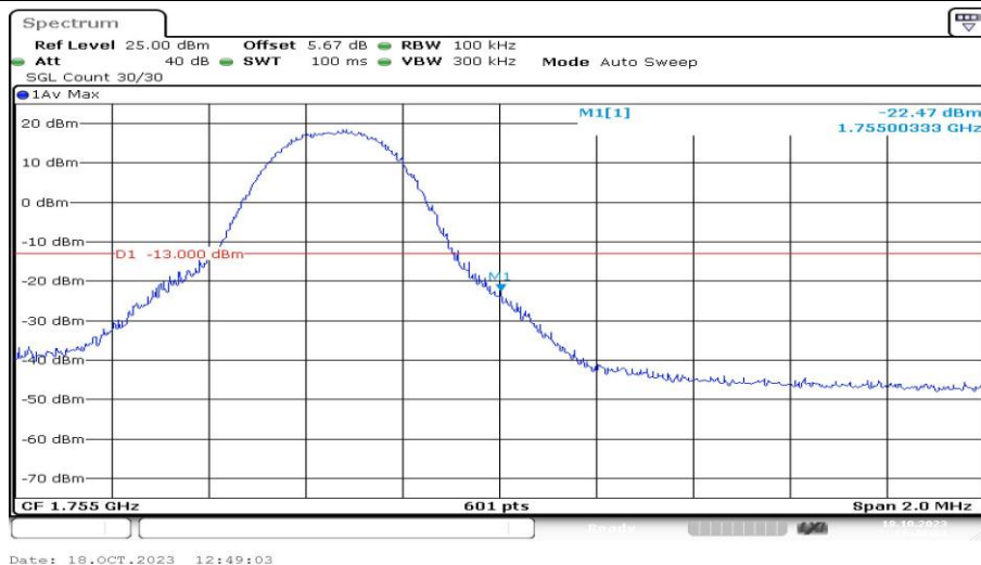
Band4-5MHz-16QAM-20375-1RB#24-PASS
