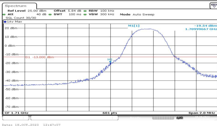
Band4-5MHz-QPSK-19975-1RB#0-PASS
