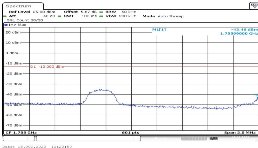
Band4-3MHz-QPSK-20385-1RB#0-PASS
