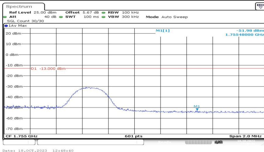
Band4-5MHz-16QAM-20375-1RB#0-PASS
