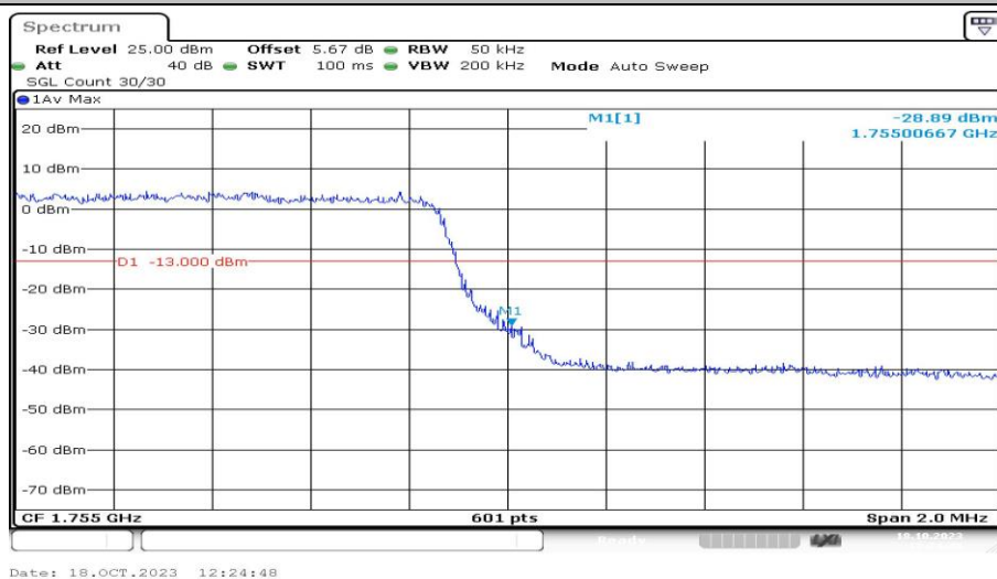
Band4-3MHz-16QAM-20385-15RB#0-PASS
