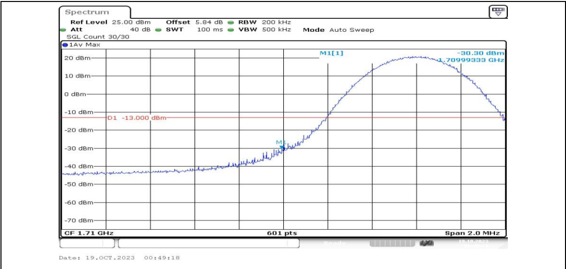
Band4-10MHz-16QAM-20000-1RB#0-PASS
