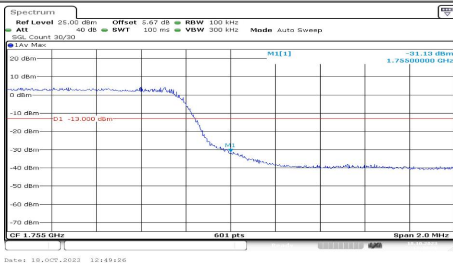
Band4-5MHz-16QAM-20375-25RB#0-PASS
