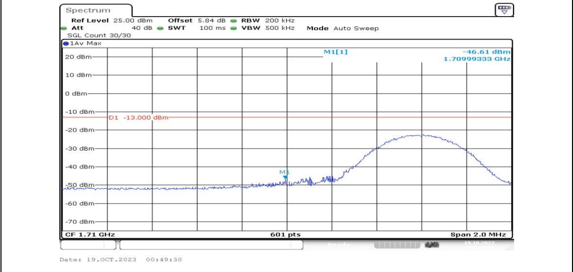
Band4-10MHz-16QAM-20000-1RB#49-PASS
