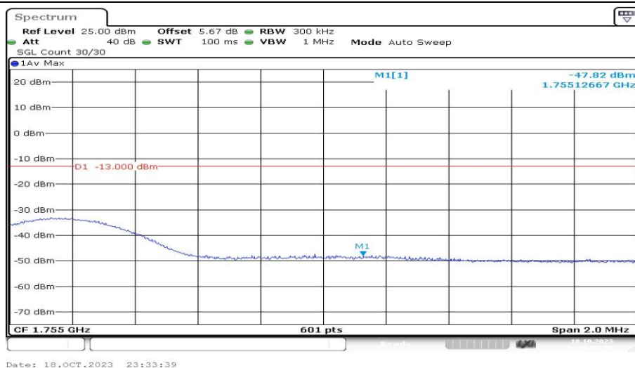
Band4-15MHz-QPSK-20325-1RB#0-PASS
