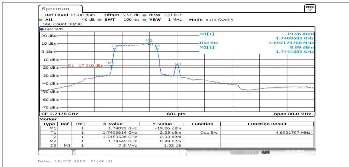
Band4-15MHz-16QAM-20325-25RB#0-PASS
