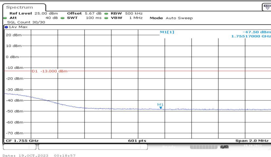
Band4-20MHz-QPSK-20300-1RB#0-PASS
