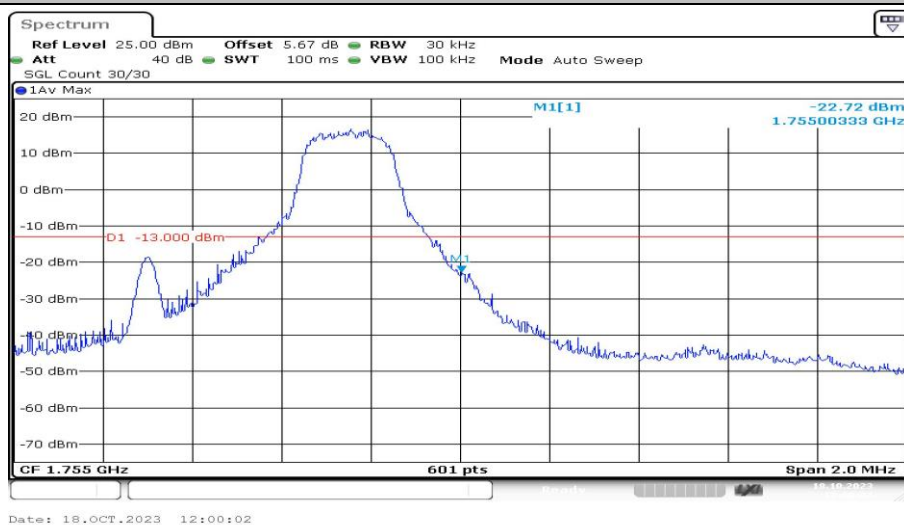
Band4-1.4MHz-QPSK-20393-1RB#5-PASS
