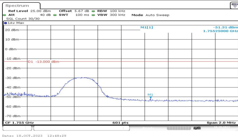
Band4-5MHz-QPSK-20375-1RB#0-PASS
