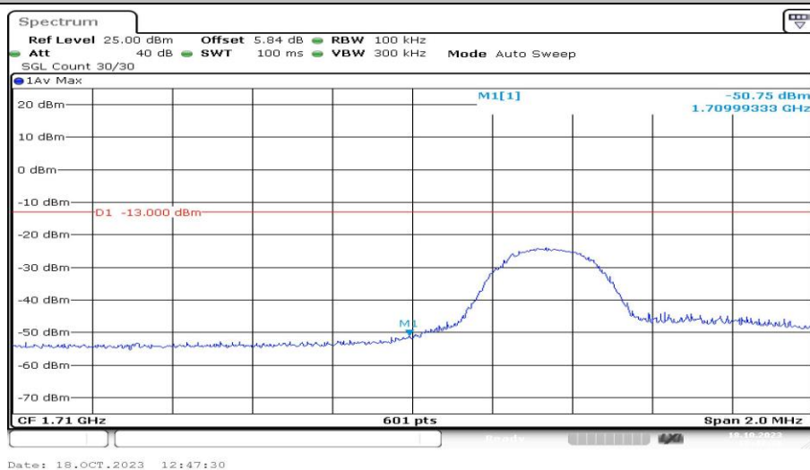
Band4-5MHz-QPSK-19975-1RB#24-PASS
