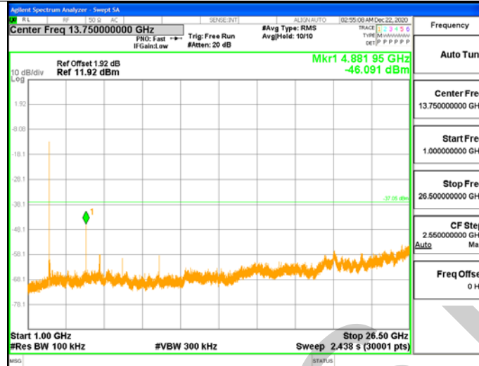
2DH1_Ant1_2480_0~Reference
