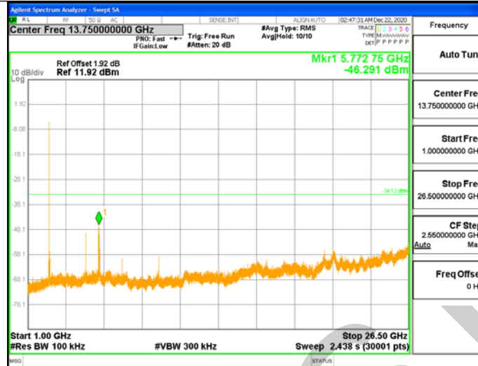
DH1_Ant1_2480_0~Reference
