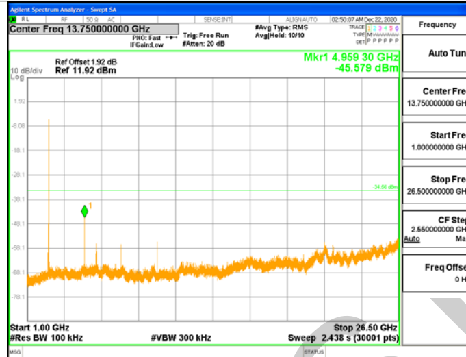
2DH1_Ant1_2402_0~Reference
