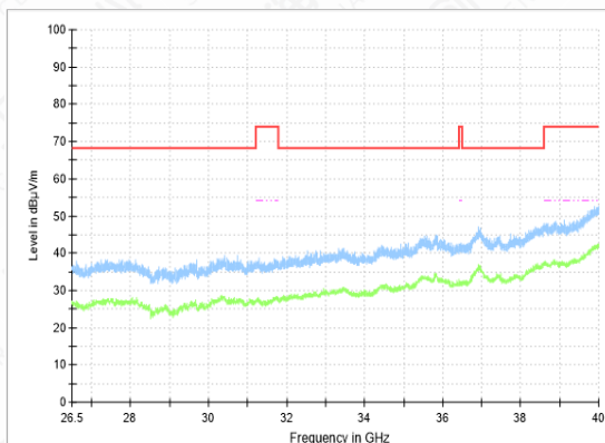
RSE-11N-CH157-26.5GHz-40GHz
