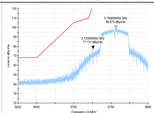
BANDEGE-11N(40M)-CH151-PK
