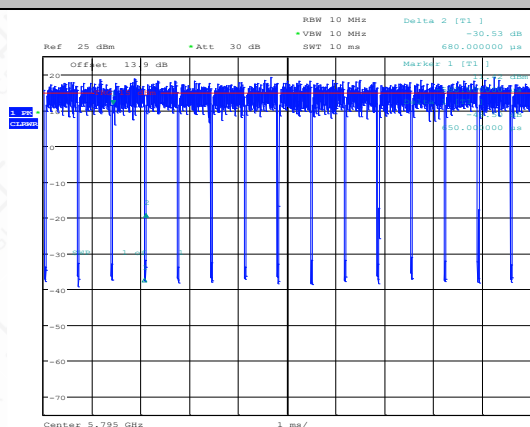
NTNV-11N40SISO-Ant1-5795
