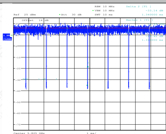
NTNV-11AC20SISO-Ant1-5825
