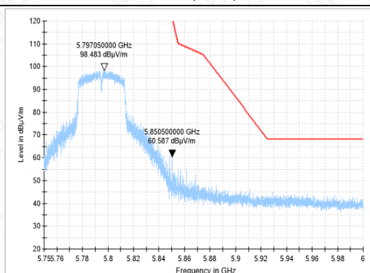
BANDEGE-11N(40M)-CH159-PK
