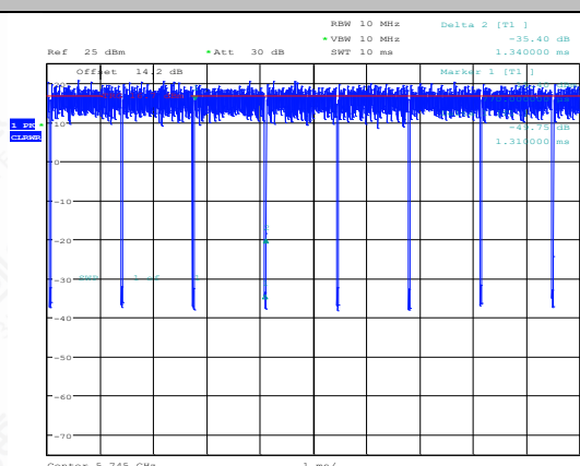
NTNV-11AC20SISO-Ant1-5745
