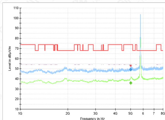
RSE-11AC(40M)-CH151-1GHz-8GHz
