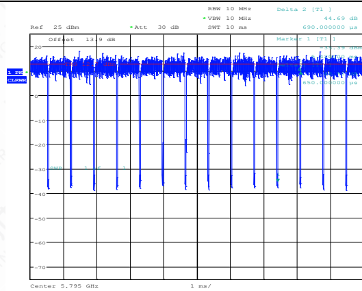
NTNV-11AC40SISO-Ant1-5795
