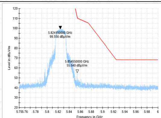
BANDEGE-11N(40M)-CH159-PK
