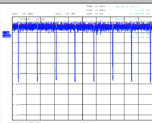
NTNV-11AC20SISO-Ant1-5785
