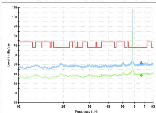
RSE-11N-CH157-1GHz-8GHz
