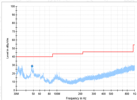
RSE-11N(40M)-CH151-30MHz-1GHz
