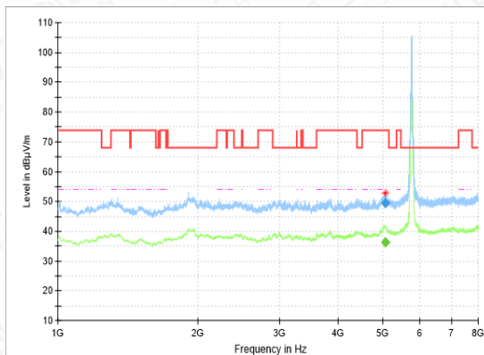
RSE-11N(40M)-CH151-1GHz-8GHz
