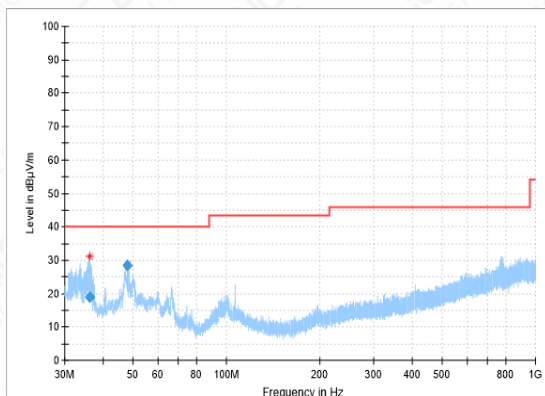
RSE-11AC(40M)-CH151-30MHz-1GHz
