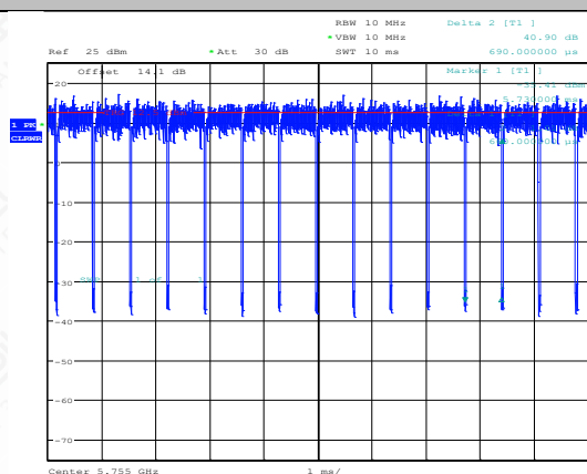
NTNV-11AC40SISO-Ant1-5755
