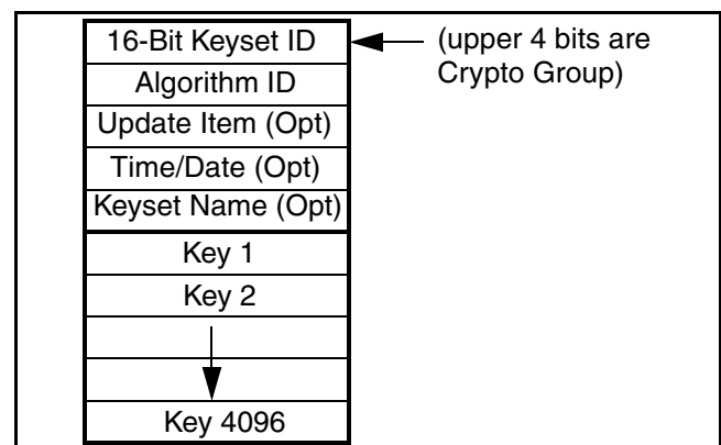
Figure 11-2 Keyset Diagram
