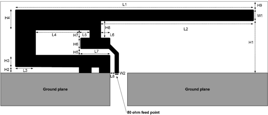
Figure 1-1. IFA Dimensions
