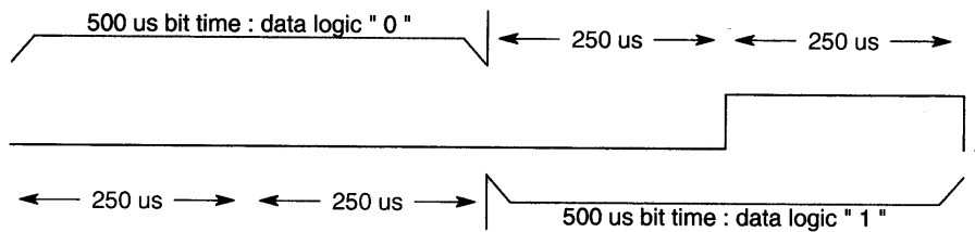
Figure 1 – Bit Timing
