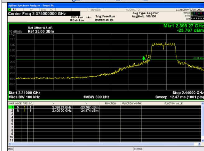
Out Of Band Emission IEEE 802.11g_Channel 1_20MHz_Antenna 2
