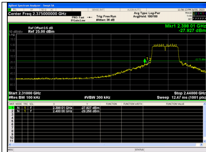
Out Of Band Emission IEEE 802.11n_Channel 1_20MHz_Antenna 2
