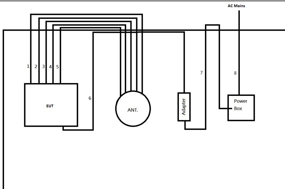
Test Setup Diagram - Radiated Test (WiFi A)
