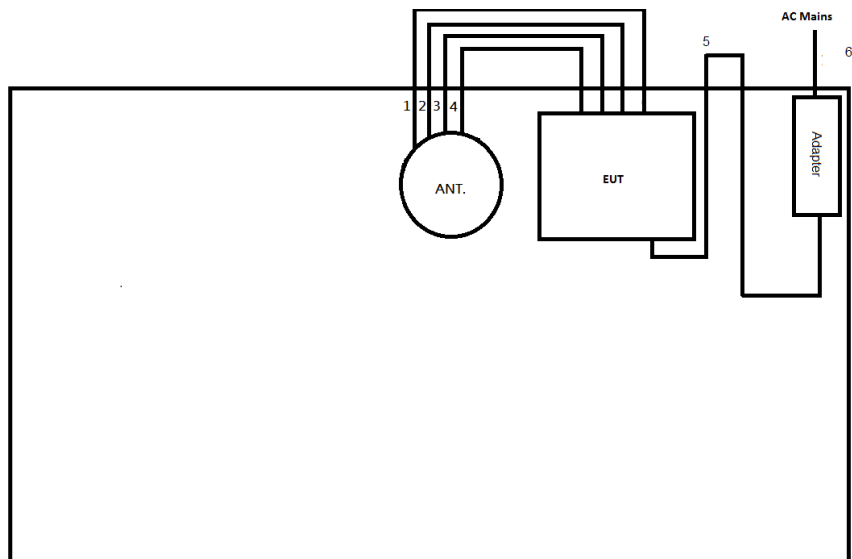
Test Setup Diagram – AC Line Conducted Emission Test (WiFi B)
