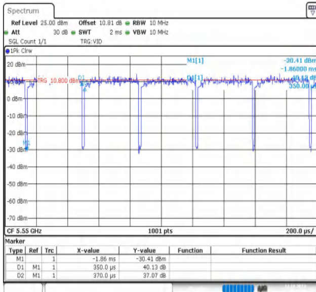
NTVN-11AC40MIMO-Ant1-5550
