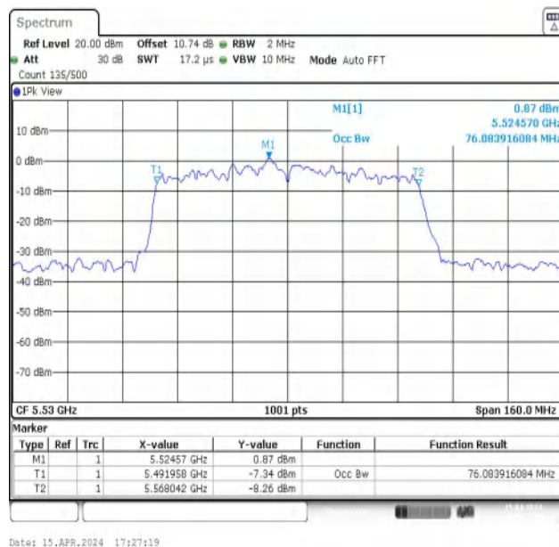
11AC80MIMO-Ant2-5530
