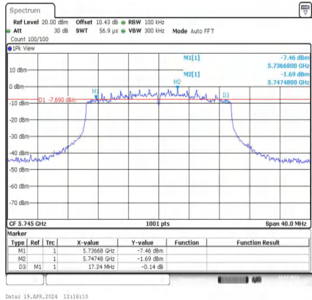
11AX20MIMO-Ant2-5745-PASS
