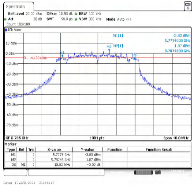
11N20MIMO-Ant2-5785-PASS
