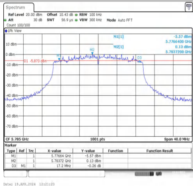
11AX20MIMO-Ant2-5785-PASS
