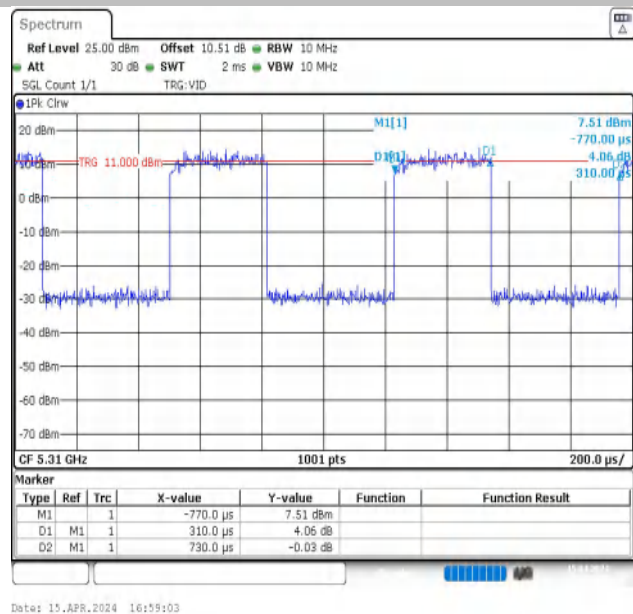
NTNV-11N40MIMO-Ant2-5310
