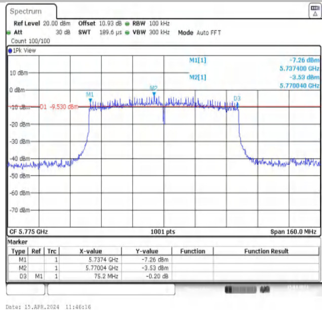
11AC80MIMO-Ant2-5775-PASS
