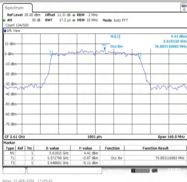
11AC80MIMO-Ant1-5610
