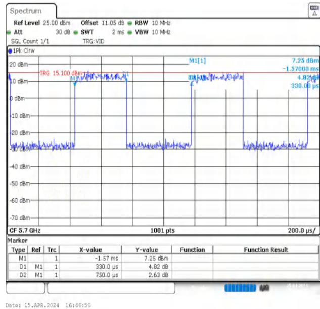
NTNV-11N20MIMO-Ant2-5700
