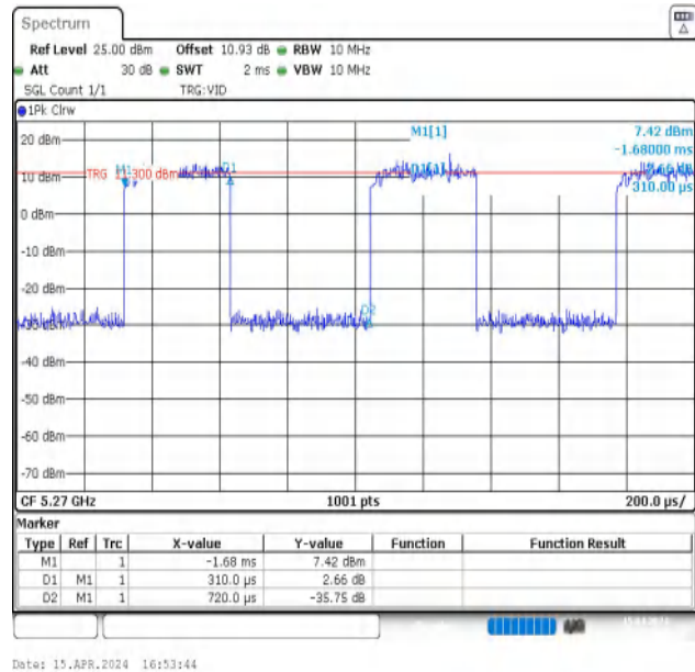
NTNV-11N40MIMO-Ant2-5270
