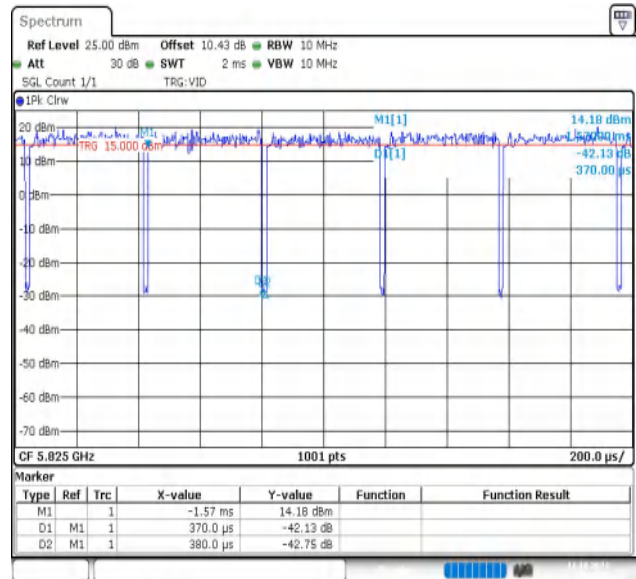
NTVN-11AC20MIMO-Ant2-5825
