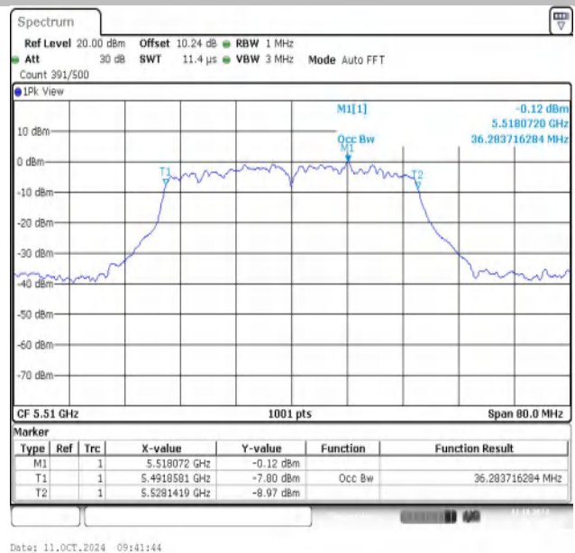
11AC40MIMO-Ant2-5510
