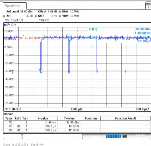
NTNV-11AC20MIMO-Ant2-5180
