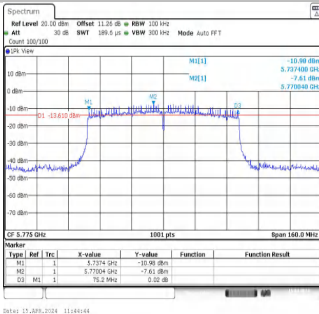
11AC80MIMO-Ant1-5775-PASS
