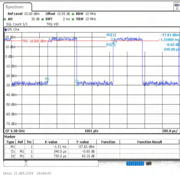
NTNV-11N20MIMO-Ant2-5580
