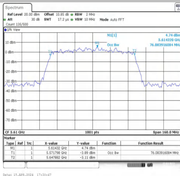
11AC80MIMO-Ant2-5610
