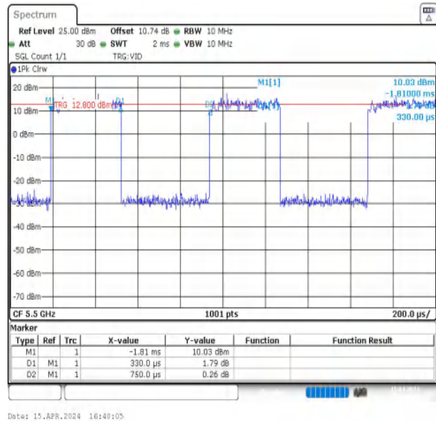
NTNV-11N20MIMO-Ant2-5500
