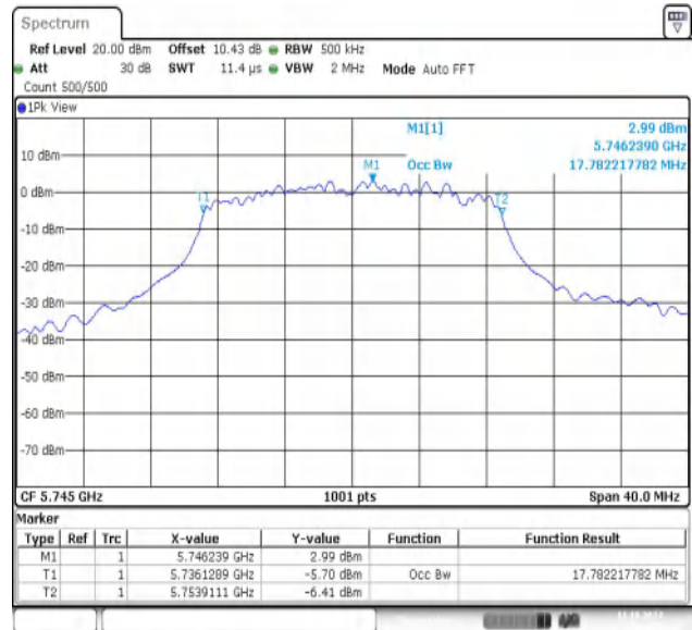
11AC20MIMO-Ant2-5745
