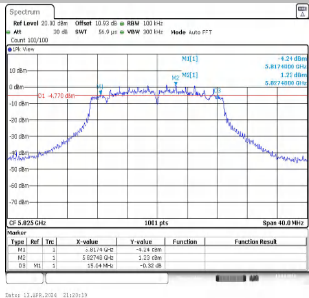
11N20MIMO-Ant2-5825-PASS
