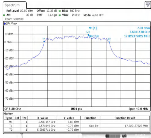
11AC20MIMO-Ant2-5580
