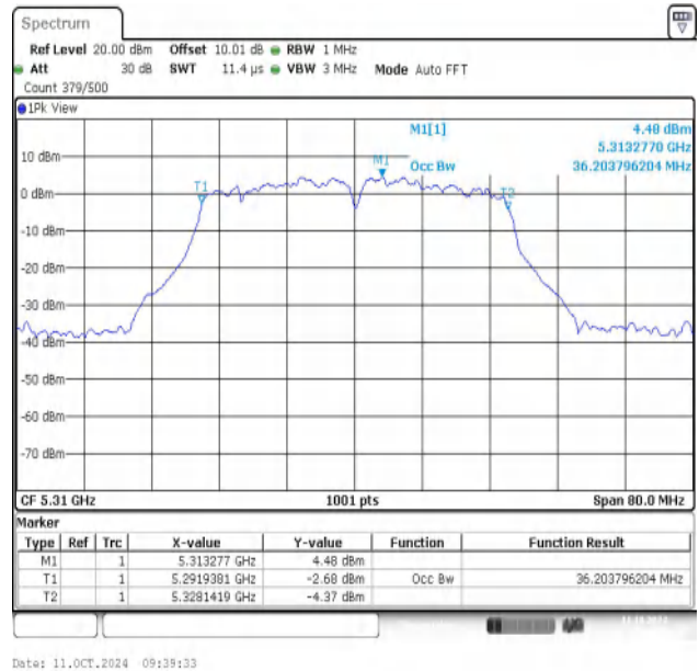
11AC40MIMO-Ant2-5310
