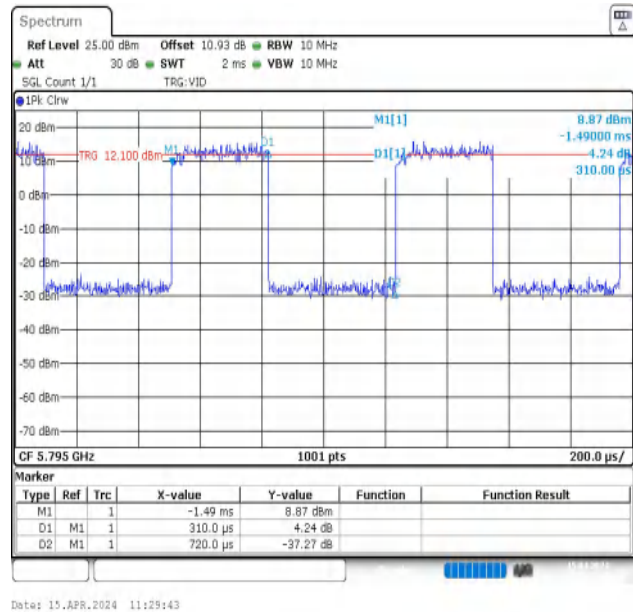
NTNV-11N40MIMO-Ant2-5795
