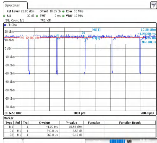
NTVN-11AC40MIMO-Ant2-5550
