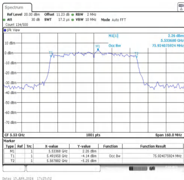
11AC80MIMO-Ant1-5530
