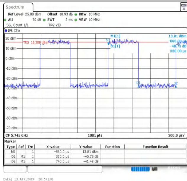
NTNV-11N20MIMO-Ant2-5745
