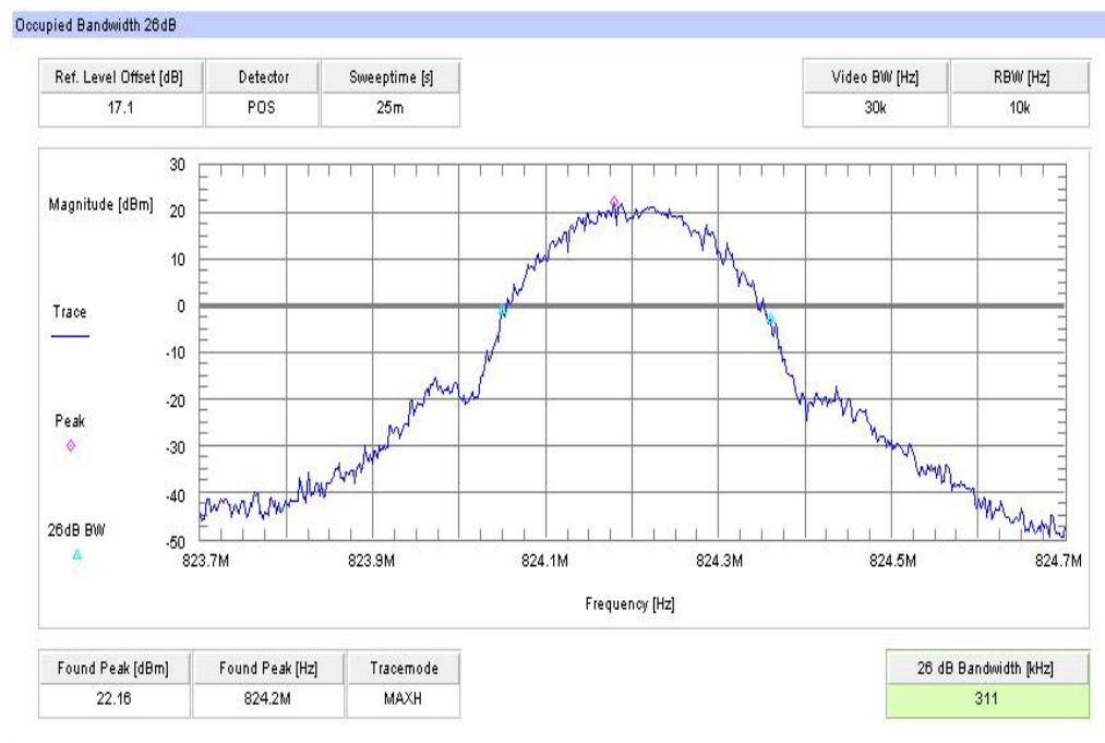
Plot 8: Channel 128 (-26 dBc BW) - 8-PSK
