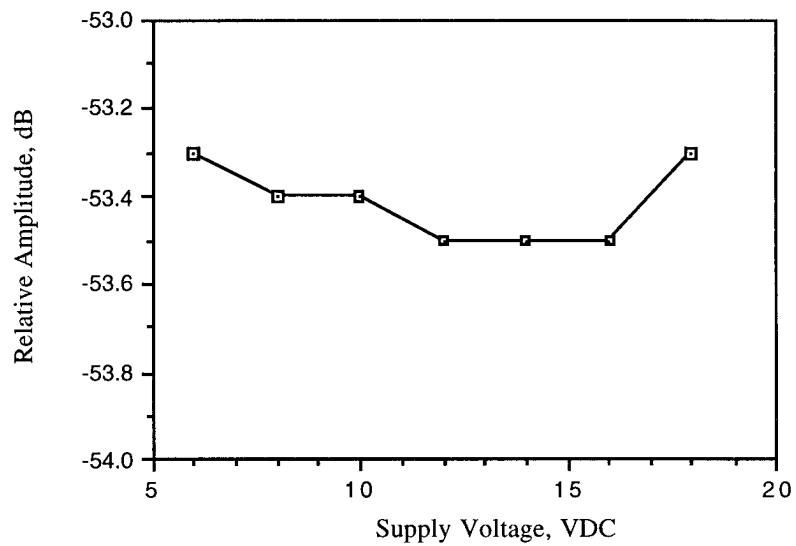
Figure 6.2. Relative emission at 651.4 MHz vs. supply voltage.
