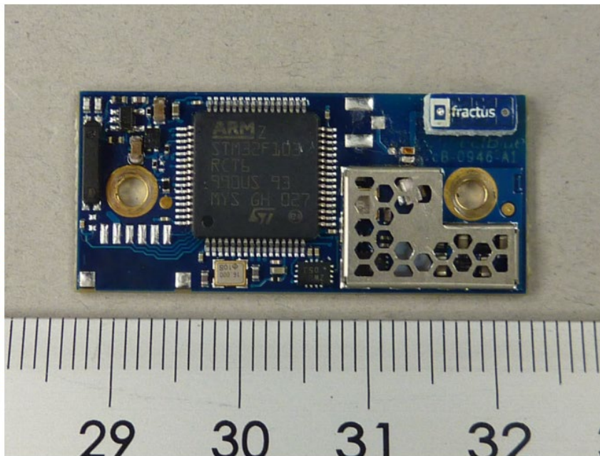
111592_i.JPG: CB-0946 with internal antenna, PCB, top view
