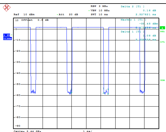
Duty Cycle 1Mbps
