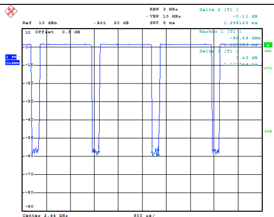
Duty Cycle 2Mbps
