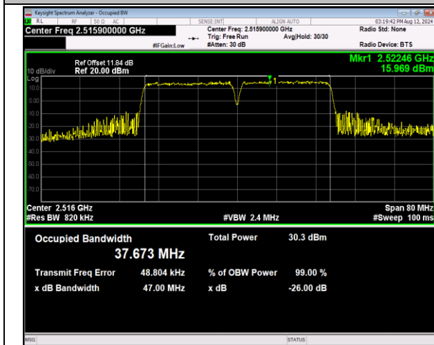
41-41-20MHz-20MHz-16QAM-16QAM-39750-39948-100RB#0-100RB#0-PASS
