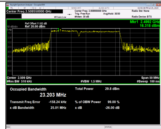
41-41-10MHz-15MHz-64QAM-64QAM-39703-39823-50RB#0-75RB#0-PASS
