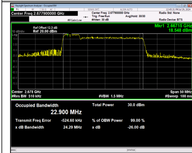
41-41-5MHz-20MHz-64QAM-64QAM-41373-41490-25RB#0-100RB#0-PASS
