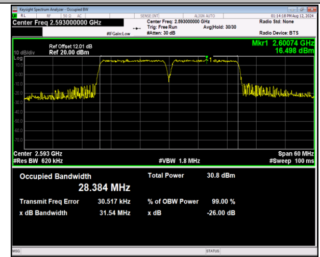
41-41-15MHz-15MHz-QPSK-QPSK-40545-40695-75RB#0 -75RB#0-PASS
