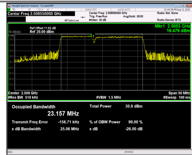
41-41-10MHz-15MHz-QPSK-QPSK-39703-39823-50RB#0-75RB#0-PASS
