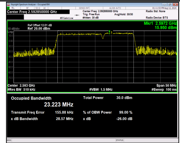
41-41-15MHz-10MHz-16QAM-16QAM-40571-40691-75RB #0-50RB#0-PASS
