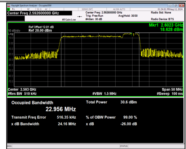
41-41-20MHz-5MHz-QPSK-QPSK-40595-40712-100RB#0 -25RB#0-PASS
