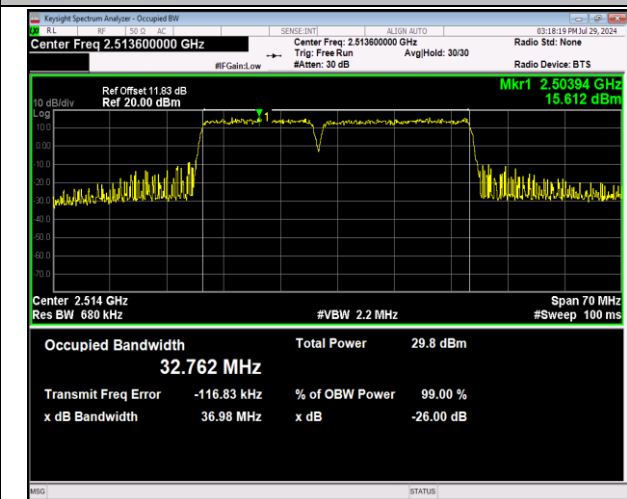
41-41-15MHz-20MHz-64QAM-64QAM-39728-39899-75RB #0-100RB#0-PASS
