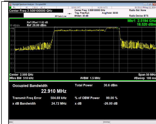
41-41-20MHz-5MHz-QPSK-QPSK-39750-39867-100RB#0 -25RB#0-PASS
