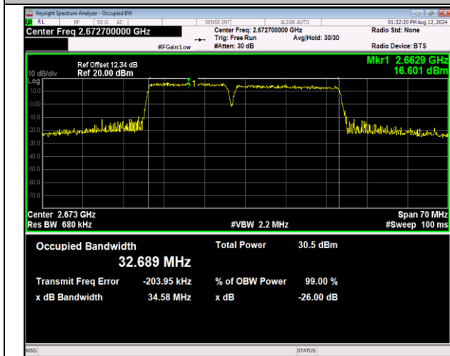
41-41-15MHz-20MHz-16QAM-16QAM-41319-41490-75RB #0-100RB#0-PASS
