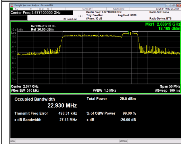
41-41-20MHz-5MHz-64QAM-64QAM-41440-41557-100RB #0-25RB#0-PASS
