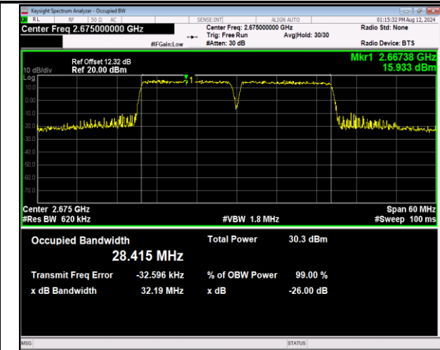
41-41-15MHz-15MHz-16QAM-16QAM-41365-41515-75RB #0-75RB#0-PASS
