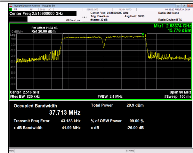
41-41-20MHz-20MHz-64QAM-64QAM-39750-39948-100RB#0-100RB#0-PASS
