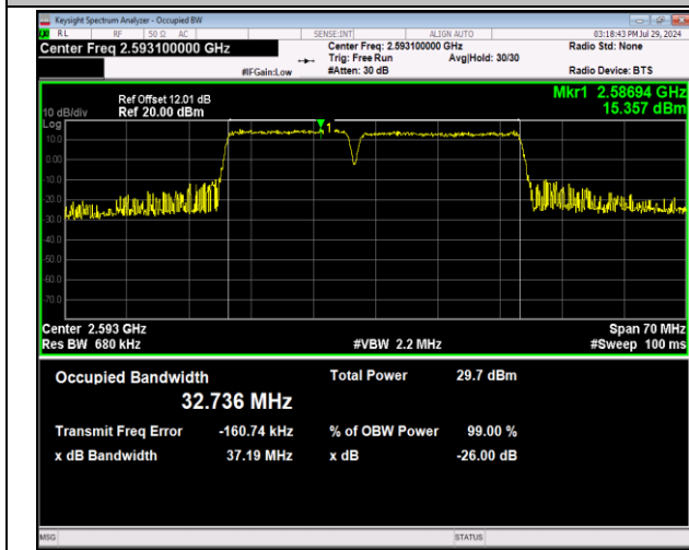
41-41-15MHz-20MHz-64QAM-64QAM-40523-40694-75RB #0-100RB#0-PASS
