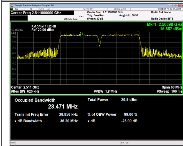
41-41-15MHz-15MHz-64QAM-64QAM-39725-39875-75RB #0-75RB#0-PASS
