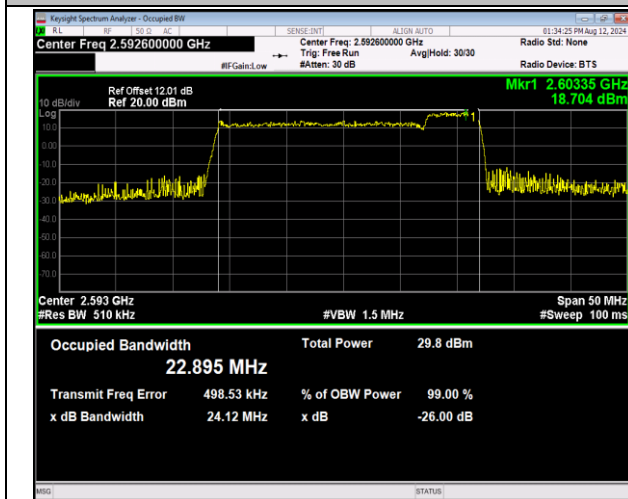
41-41-20MHz-5MHz-16QAM-16QAM-40595-40712-100RB #0-25RB#0-PASS
