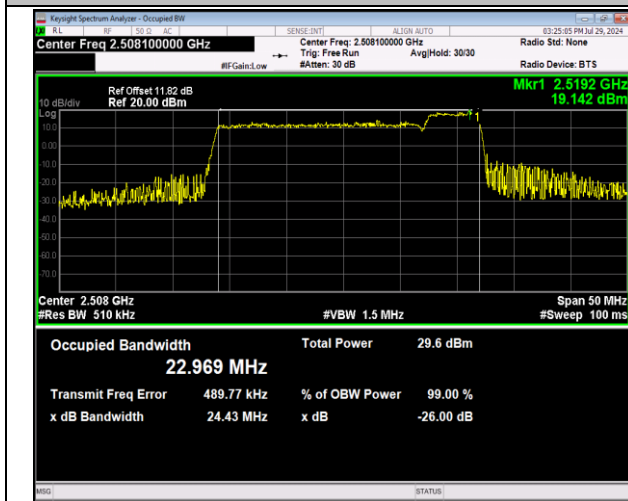
41-41-20MHz-5MHz-64QAM-64QAM-39750-39867-100RB #0-25RB#0-PASS
