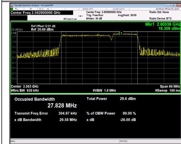
41-41-20MHz-10MHz-64QAM-64QAM-40571-40715-100RB#0-50RB#0-PASS
