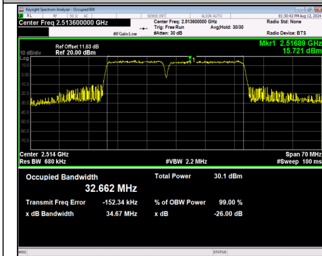
41-41-15MHz-20MHz-16QAM-16QAM-39728-39899-75RB #0-100RB#0-PASS
