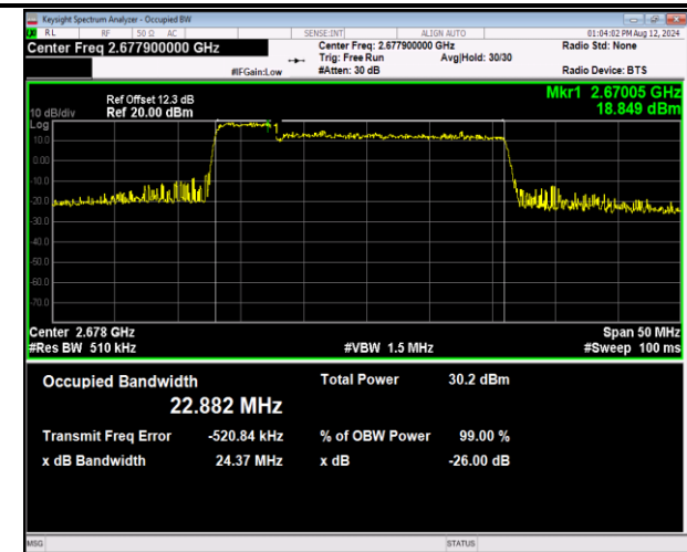
41-41-5MHz-20MHz-16QAM-16QAM-41373-41490-25RB#0-100RB#0-PASS
