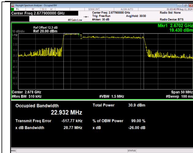
41-41-5MHz-20MHz-QPSK-QPSK-41373-41490-25RB#0-100RB#0-PASS
