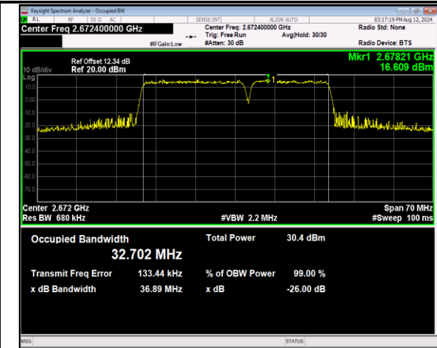
41-41-20MHz-15MHz-16QAM-16QAM-41341-41512-100RB#0-75RB#0-PASS
