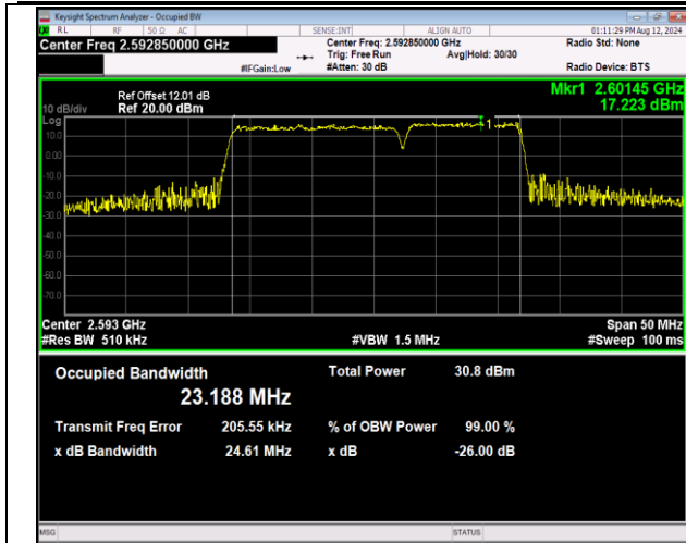
41-41-15MHz-10MHz-QPSK-QPSK-40571-40691-75RB#0 -50RB#0-PASS
