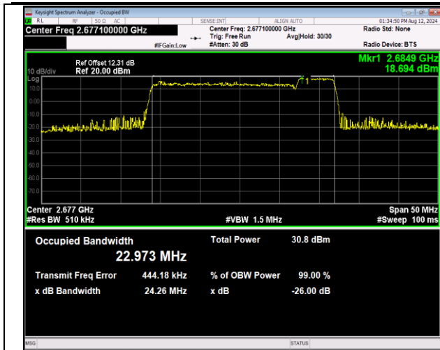
41-41-20MHz-5MHz-QPSK-QPSK-41440-41557-100RB#0 -25RB#0-PASS
