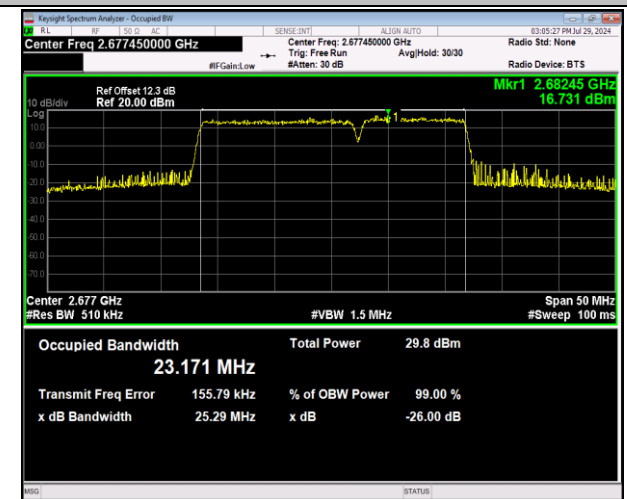
41-41-15MHz-10MHz-64QAM-64QAM-41417-41537-75RB #0-50RB#0-PASS
