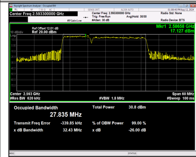
41-41-10MHz-20MHz-QPSK-QPSK-40526-40670-50RB#0 -100RB#0-PASS
