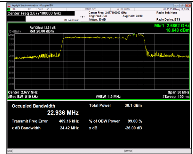
41-41-20MHz-5MHz-16QAM-16QAM-41440-41557-100RB #0-25RB#0-PASS
