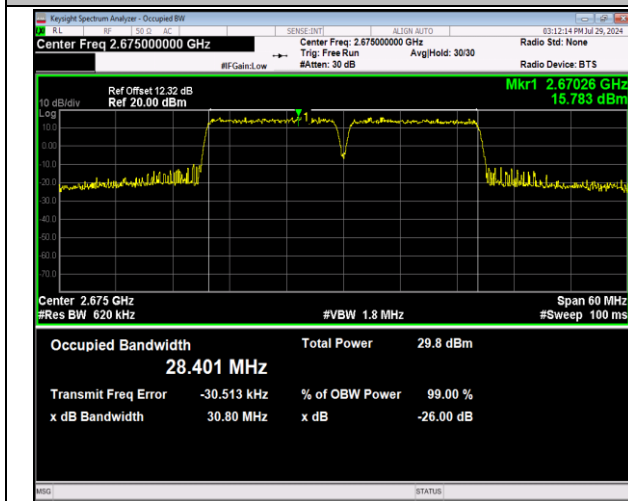
41-41-15MHz-15MHz-64QAM-64QAM-41365-41515-75RB #0-75RB#0-PASS
