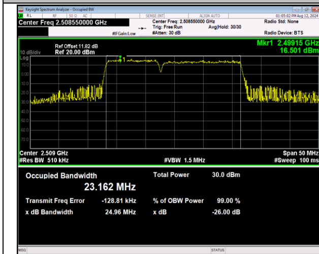
41-41-10MHz-15MHz-16QAM-16QAM-39703-39823-50RB#0-75RB#0-PASS
