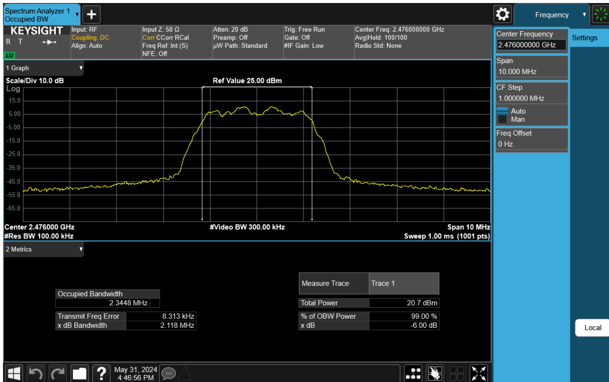
Plot 7-9. 6dB BW & 99% OBW Plot Antenna WF7 (Bluetooth (HDR4), 4Mbps, ePA – Ch. 73)
