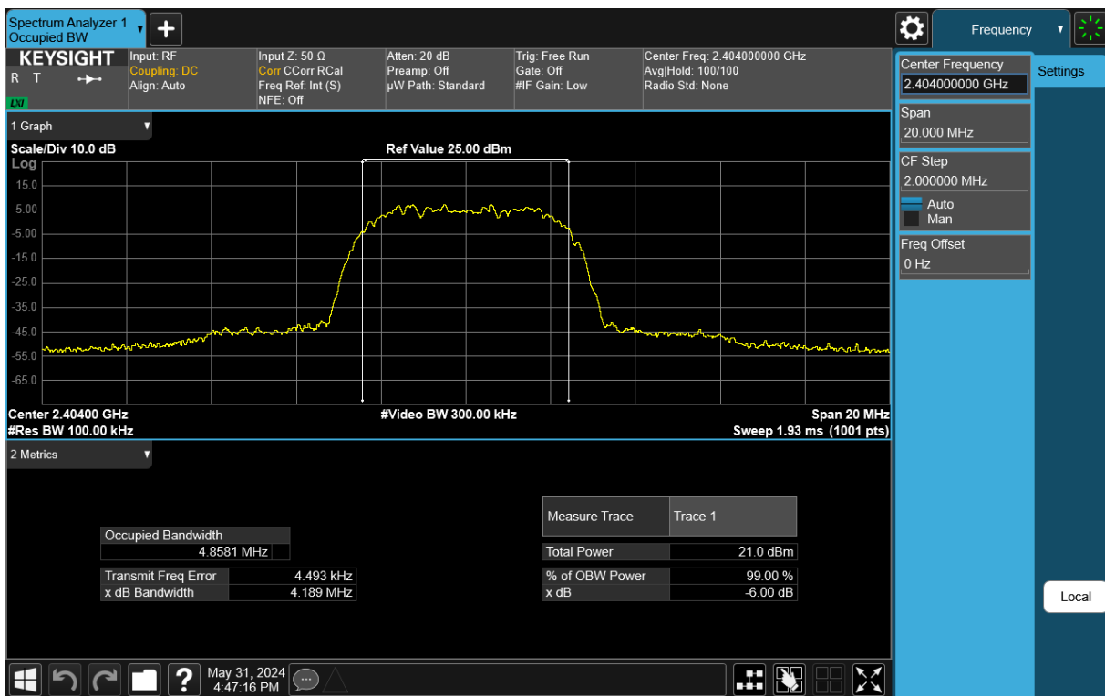
Plot 7-10. 6dB BW & 99% OBW Plot Antenna WF7 (Bluetooth (HDR8), 8Mbps, ePA – Ch. 1)
