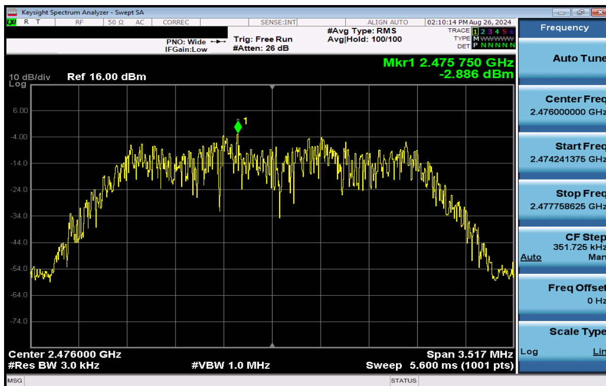
Plot 7-33. Power Spectral Density Plot Antenna WF7 (Bluetooth (HDR4), 4Mbps, ePA – Ch. 73)
