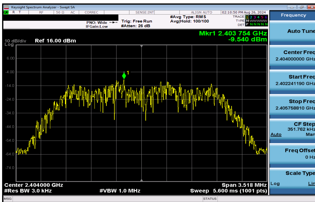
Plot 7-34. Power Spectral Density Plot Antenna WF7 (Bluetooth (HDR4), 4Mbps, iPA – Ch. 1)
