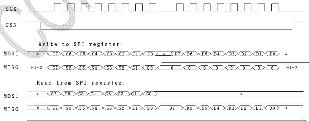
Figure 6 SPI timing
