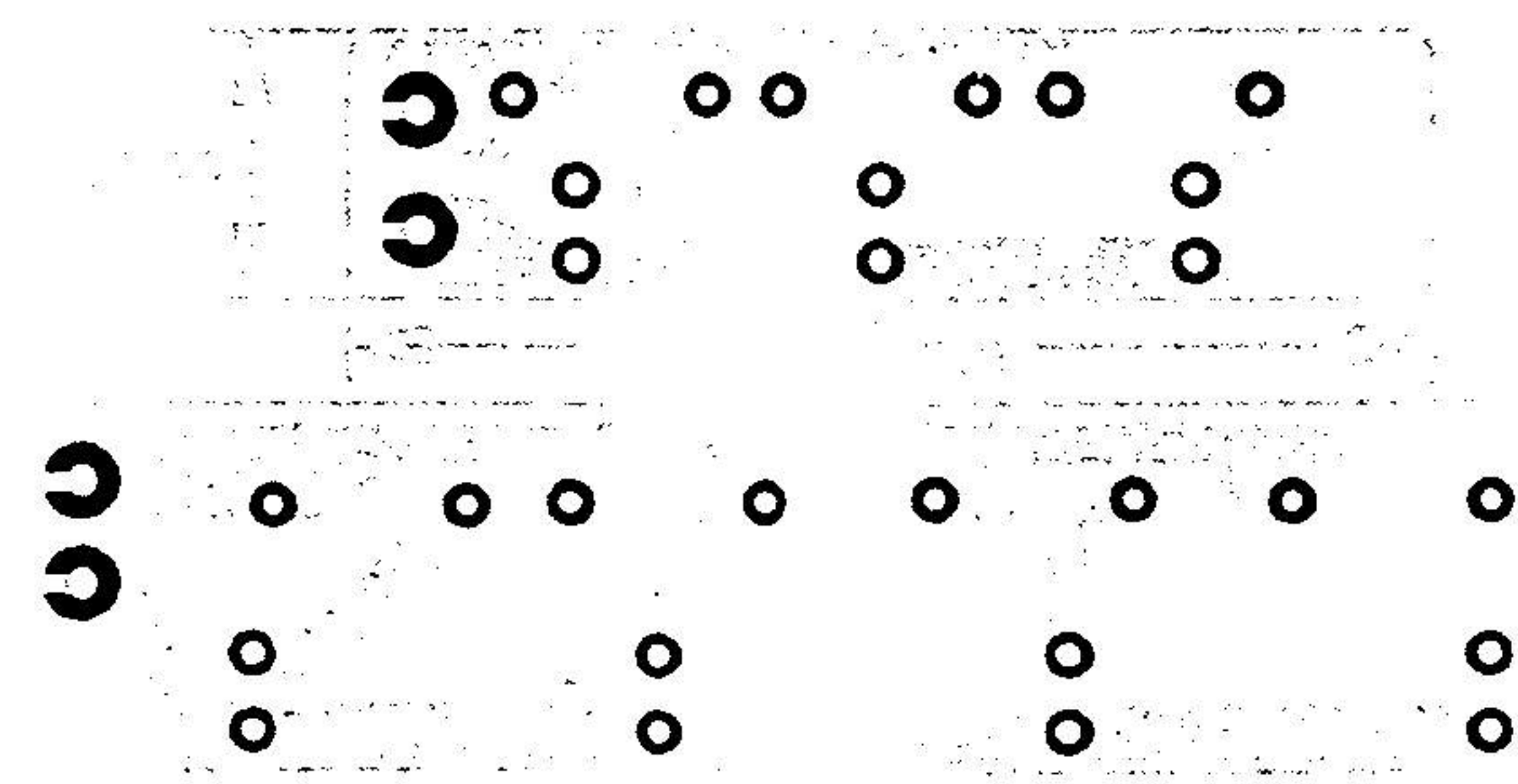
FRONE WHEEL LED(S) PCB
