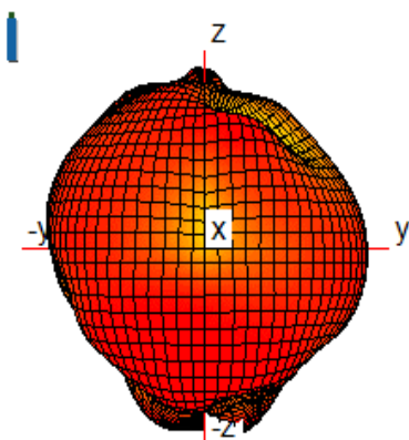
3D Antenna Pattern
