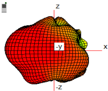
3D Antenna Pattern
