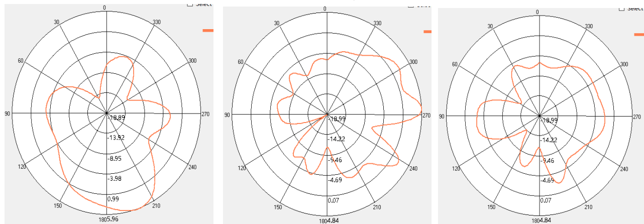
2D Antenna Pattern (X->Y;X->Z;Y->Z)
