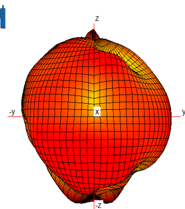
3D Antenna Pattern
