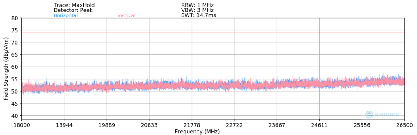
Plot 7-84. Radiated Spurious Plot above 18GHz SISO ANT1 – Half Open
