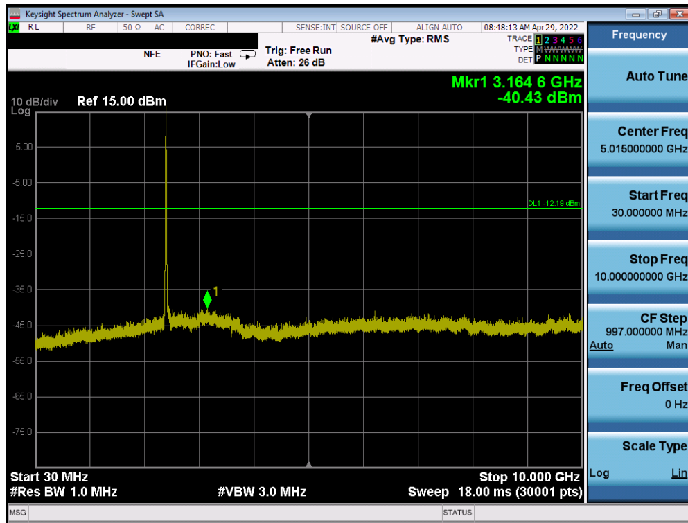
Plot 7-71. Conducted Spurious Plot SISO ANT2 (802.11b – Ch. 1)
