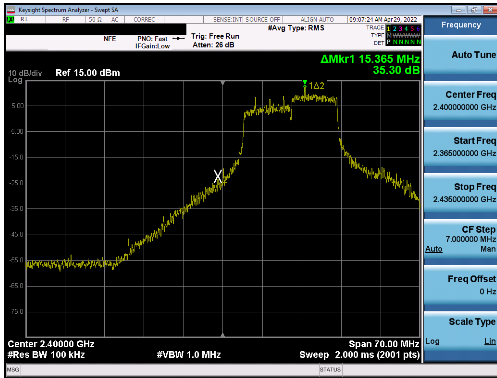
Plot 7-59. Band Edge Plot SISO ANT2 (802.11g- Ch. 1)
