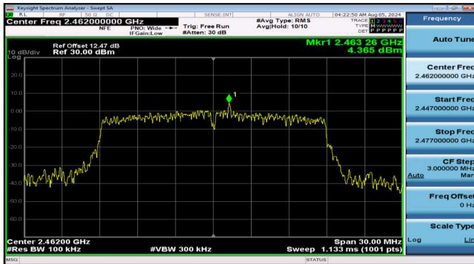
11N20SISO-Ant1-2462-0~Reference-PASS
