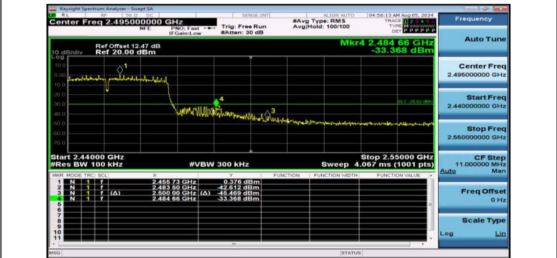
11N40SISO-Ant1-2452-PASS
