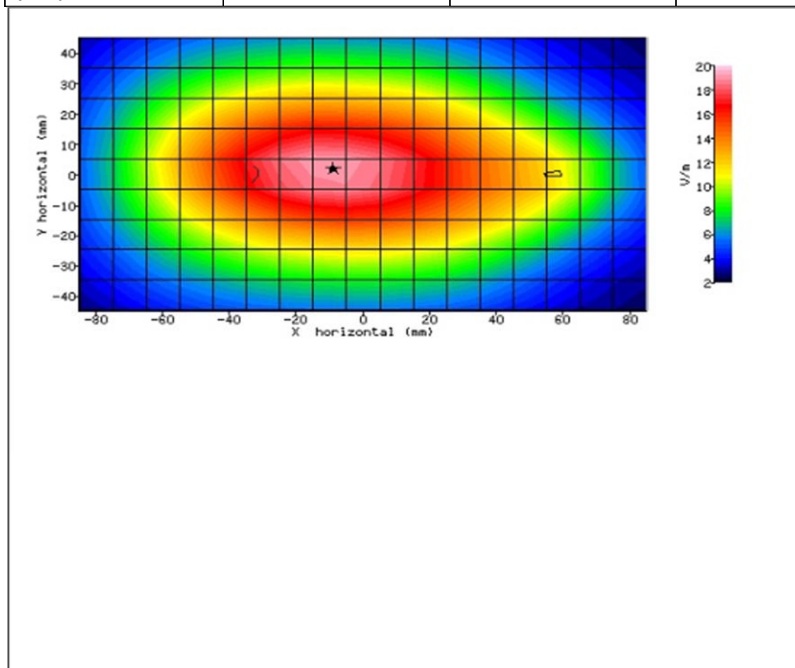
Figure 40: SAR Body Testing Results for the Sharp Smart phone at 829.0MHz.
