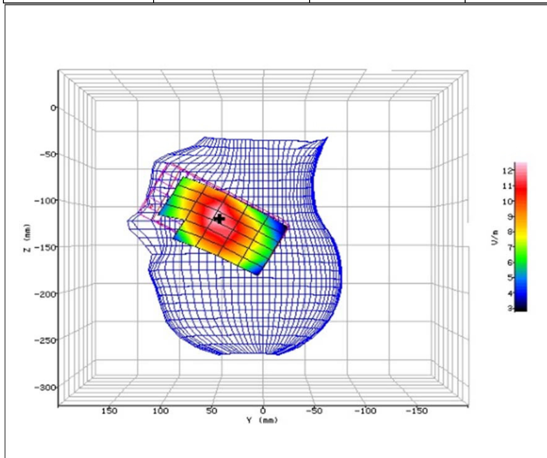
Figure 35: SAR Head Testing Results for the Sharp Smart phone at 829.0MHz.
