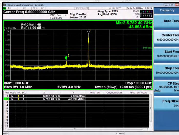
11AX40SISO-Ant1-6845-26Tone-RU17-3000~10000-PASS
