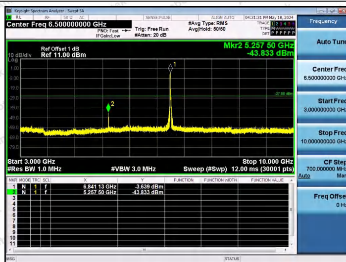
11AX40SISO-Ant1-6845-242Tone-RU61-3000~10000-PASS
