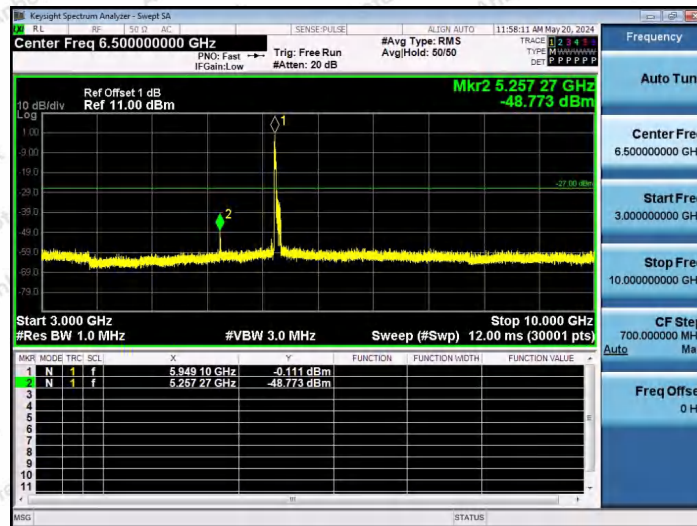
11AX80SISO-Ant1-5985-52Tone-RU37-3000~10000-PASS
