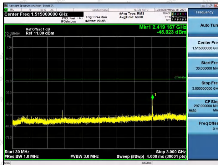
11AX80SISO-Ant1-5985-106Tone-RU53-30~3000-PASS
