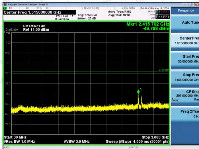
11AX40SISO-Ant1-7085-242Tone-RU61-30~3000-PASS
