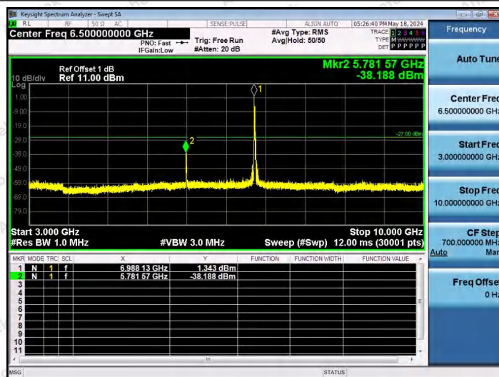
11AX40SISO-Ant1-7005-52Tone-RU37-3000~10000-PASS
