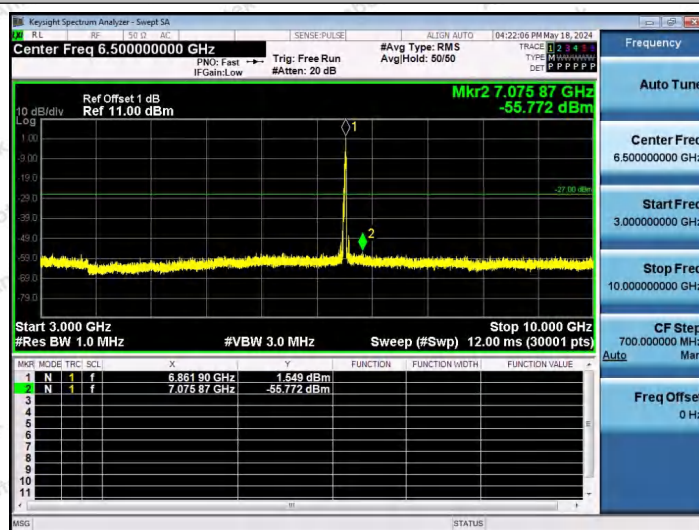
11AX40SISO-Ant1-6845-52Tone-RU44-3000~10000-PASS
