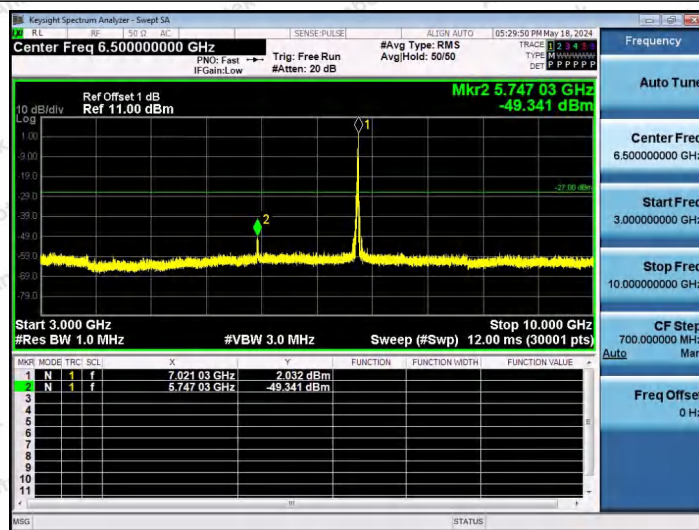
11AX40SISO-Ant1-7005-52Tone-RU44-3000~10000-PASS
