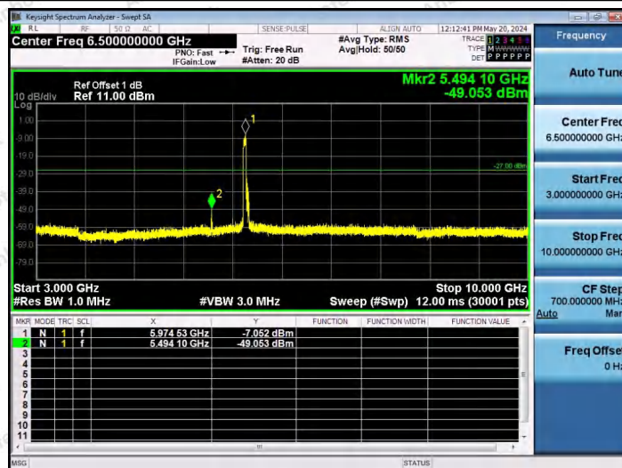
11AX80SISO-Ant1-5985-484Tone-RU65-3000~10000-PASS
