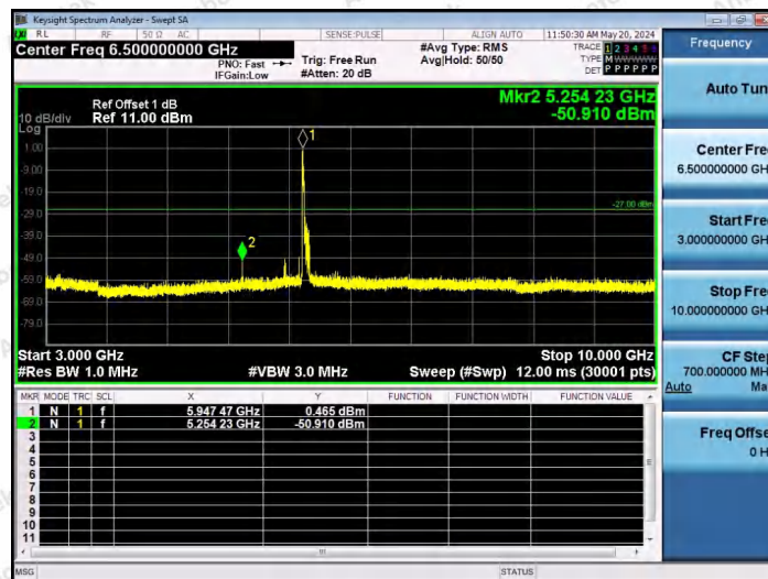
11AX80SISO-Ant1-5985-26Tone-RU0-3000~10000-PASS
