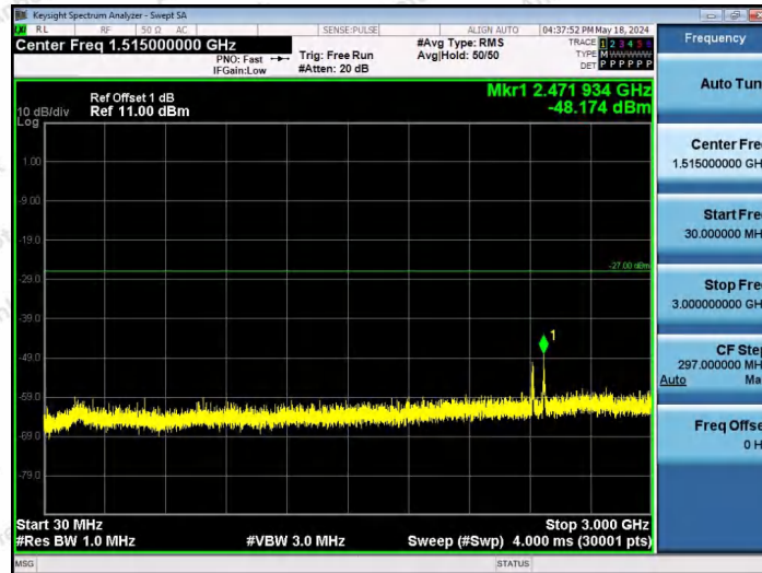
11AX40SISO-Ant1-6885-26Tone-RU0-30~3000-PASS
