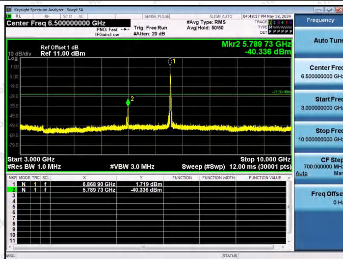
11AX40SISO-Ant1-6885-52Tone-RU37-3000~10000-PASS
