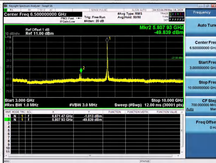
11AX40SISO-Ant1-6885-106Tone-RU53-3000~10000-PASS
