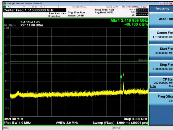
11AX40SISO-Ant1-7005-26Tone-RU0-30~3000-PASS
