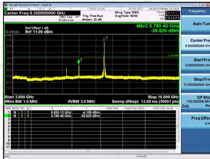
11AX40SISO-Ant1-6845-242Tone-RU62-3000~10000-PASS
