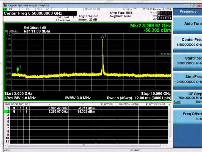
11AX40SISO-Ant1-7005-106Tone-RU53-3000~10000-PASS
