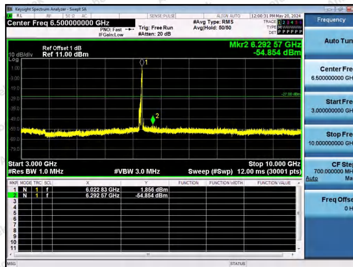
11AX80SISO-Ant1-5985-52Tone-RU52-3000~10000-PASS
