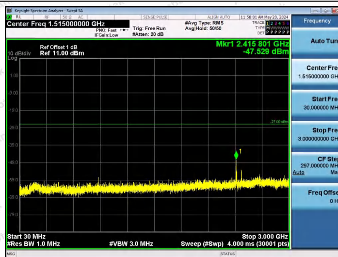
11AX80SISO-Ant1-5985-52Tone-RU37-30~3000-PASS
