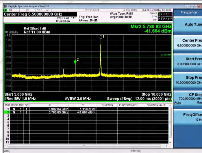
11AX40SISO-Ant1-6885-52Tone-RU44-3000~10000-PASS
