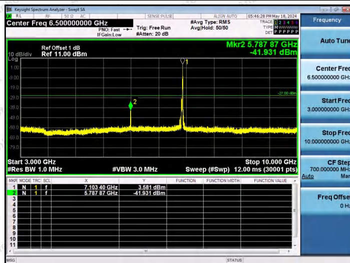
11AX40SISO-Ant1-7085-26Tone-RU17-3000~10000-PASS
