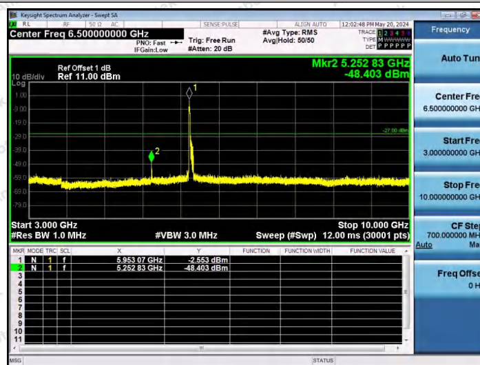
11AX80SISO-Ant1-5985-106Tone-RU53-3000~10000-PASS
