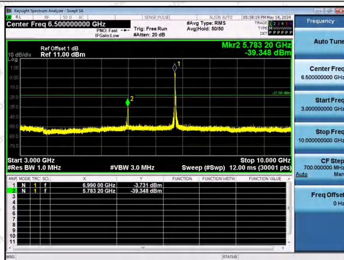
11AX40SISO-Ant1-7005-242Tone-RU61-3000~10000-PASS
