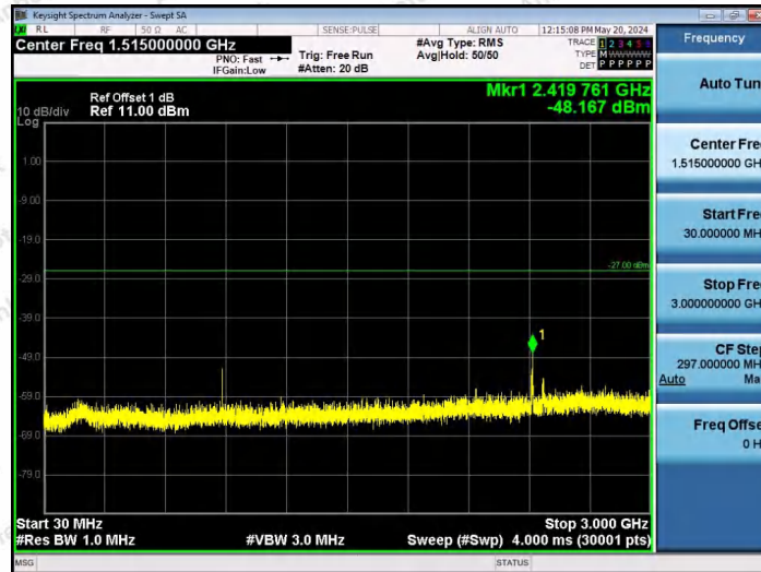
11AX80SISO-Ant1-5985-484Tone-RU66-30~3000-PASS
