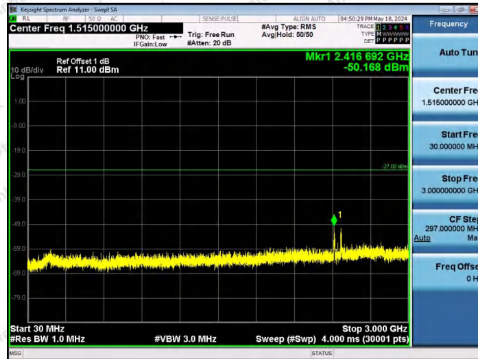
11AX40SISO-Ant1-6885-52Tone-RU44-30~3000-PASS
