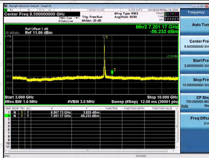
11AX40SISO-Ant1-6885-26Tone-RU0-3000~10000-PASS
