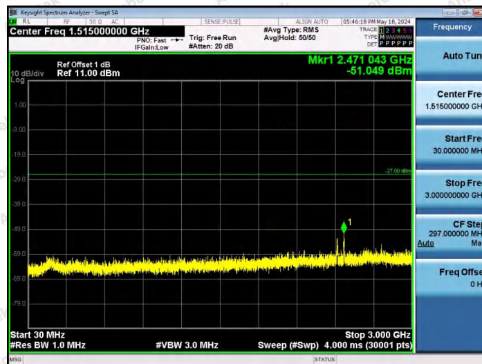
11AX40SISO-Ant1-7085-26Tone-RU17-30~3000-PASS
