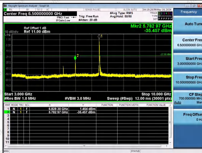
11AX40SISO-Ant1-6845-52Tone-RU37-3000~10000-PASS
