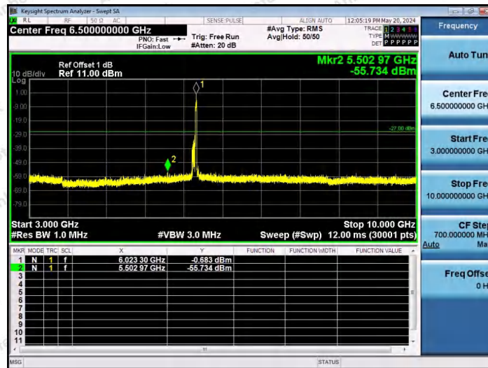
11AX80SISO-Ant1-5985-106Tone-RU60-3000~10000-PASS
