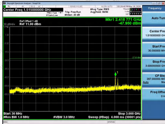
11AX40SISO-Ant1-7005-52Tone-RU44-30~3000-PASS
