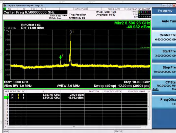
11AX80SISO-Ant1-5985-26Tone-RU36-3000~10000-PASS
