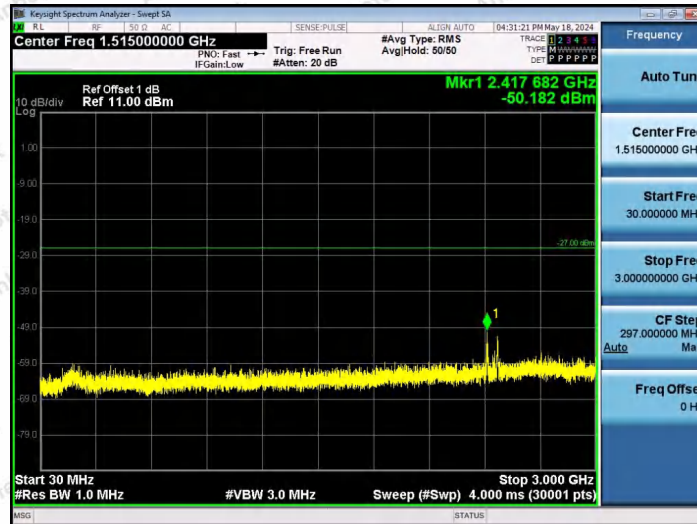
11AX40SISO-Ant1-6845-242Tone-RU61-30~3000-PASS
