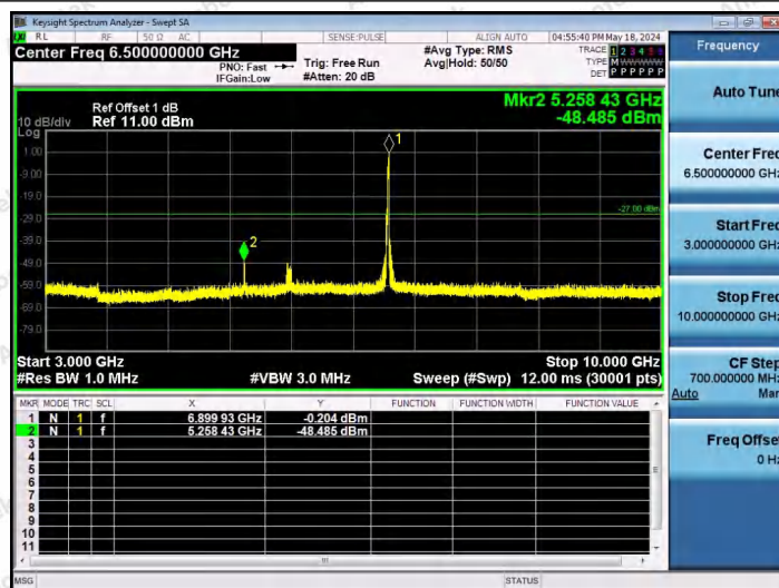
11AX40SISO-Ant1-6885-106Tone-RU56-3000~10000-PASS
