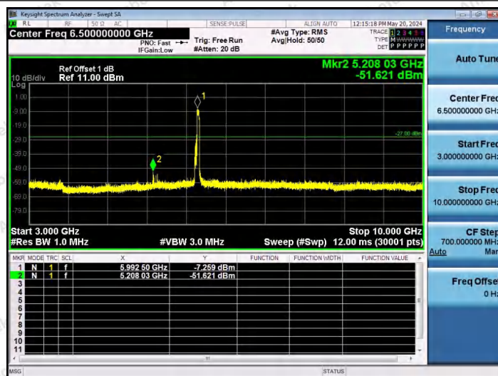
11AX80SISO-Ant1-5985-484Tone-RU66-3000~10000-PASS
