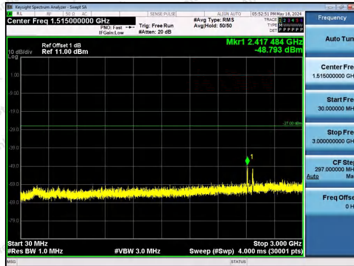
11AX40SISO-Ant1-7085-52Tone-RU44-30~3000-PASS
