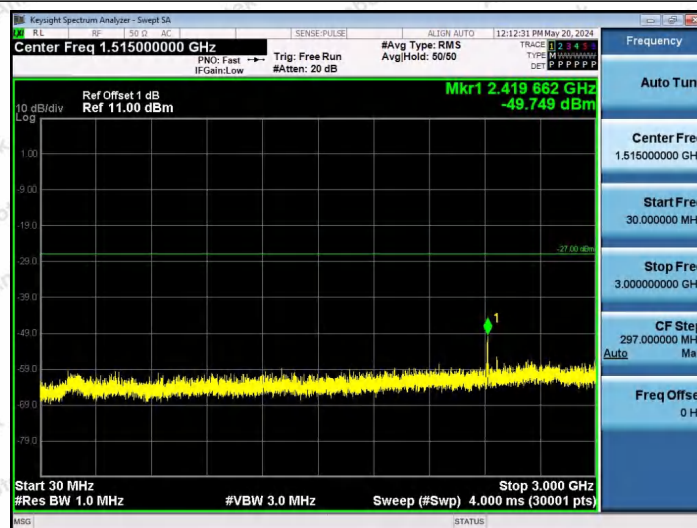
11AX80SISO-Ant1-5985-484Tone-RU65-30~3000-PASS
