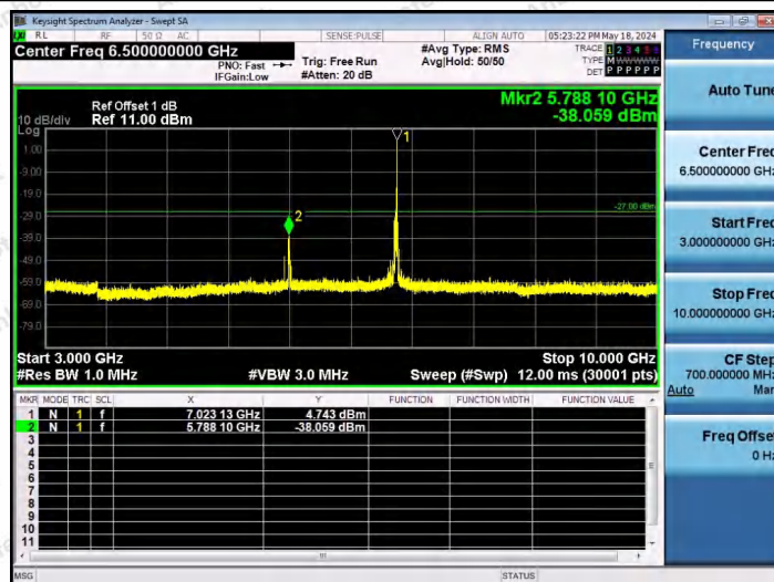
11AX40SISO-Ant1-7005-26Tone-RU17-3000~10000-PASS
