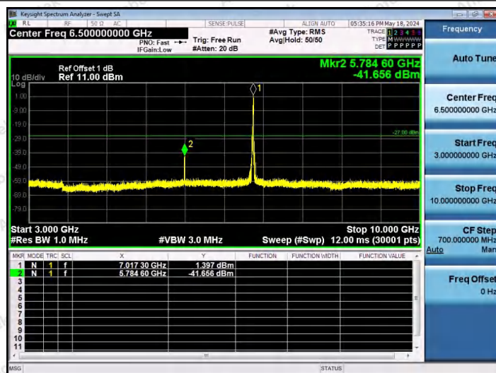
11AX40SISO-Ant1-7005-106Tone-RU56-3000~10000-PASS
