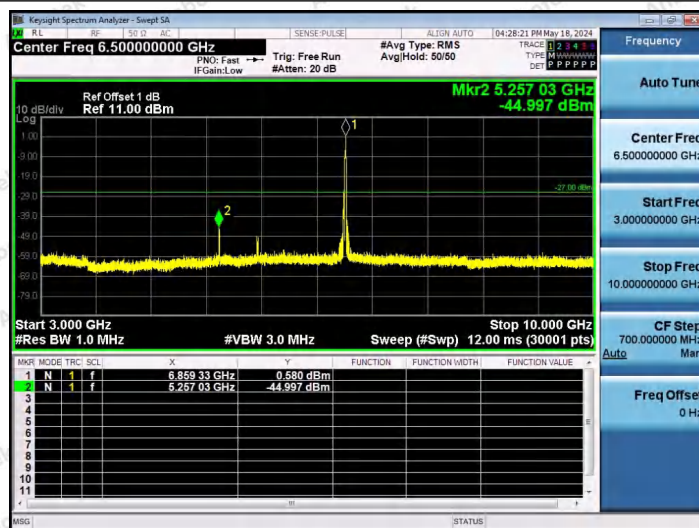
11AX40SISO-Ant1-6845-106Tone-RU56-3000~10000-PASS
