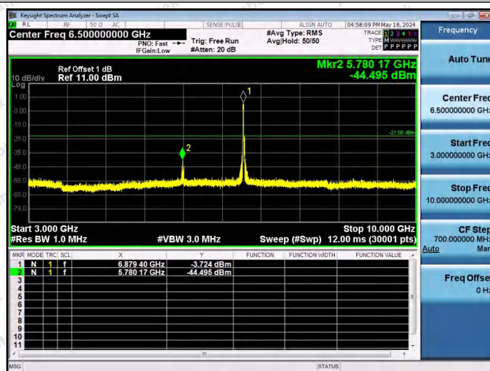
11AX40SISO-Ant1-6885-242Tone-RU61-3000~10000-PASS
