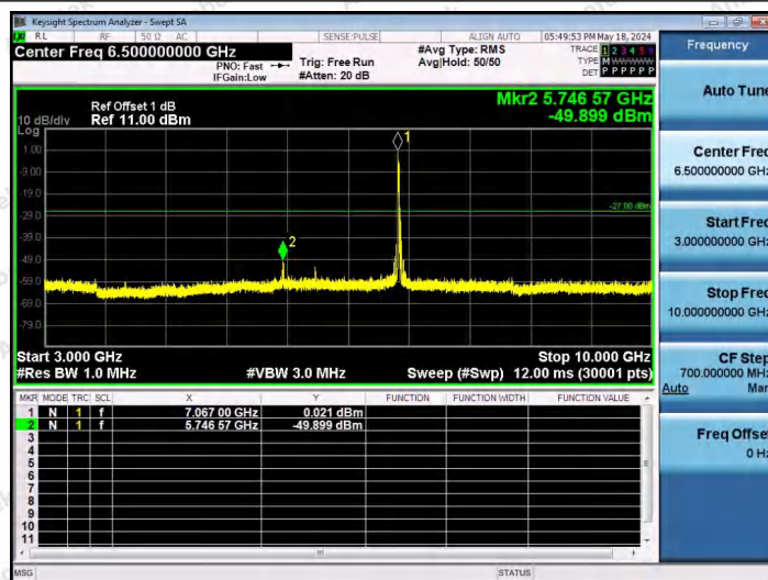
11AX40SISO-Ant1-7085-52Tone-RU37-3000~10000-PASS
