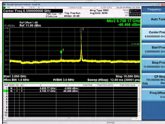
11AX40SISO-Ant1-6845-106Tone-RU53-3000~10000-PASS
