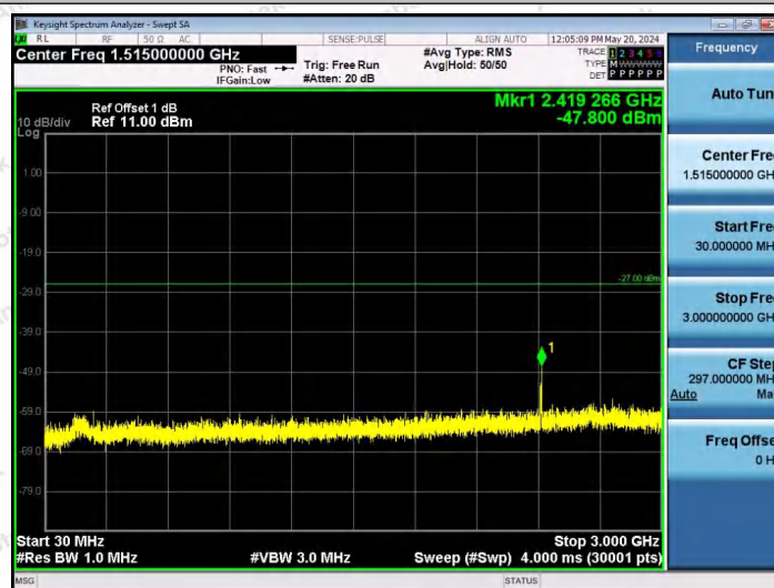
11AX80SISO-Ant1-5985-106Tone-RU60-30~3000-PASS
