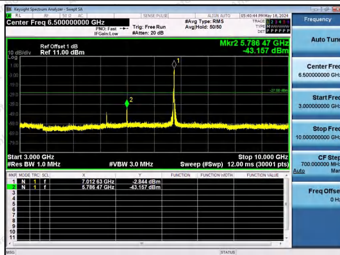
11AX40SISO-Ant1-7005-242Tone-RU62-3000~10000-PASS
