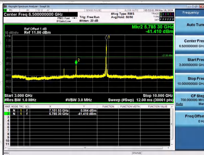
11AX40SISO-Ant1-7085-52Tone-RU44-3000~10000-PASS
