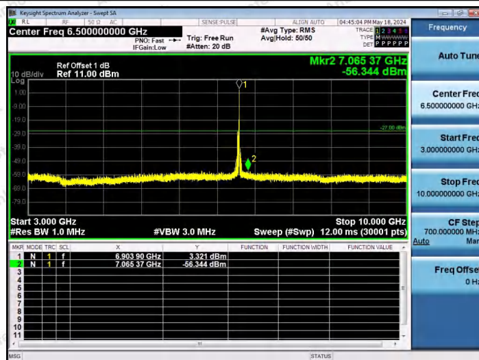
11AX40SISO-Ant1-6885-26Tone-RU17-3000~10000-PASS
