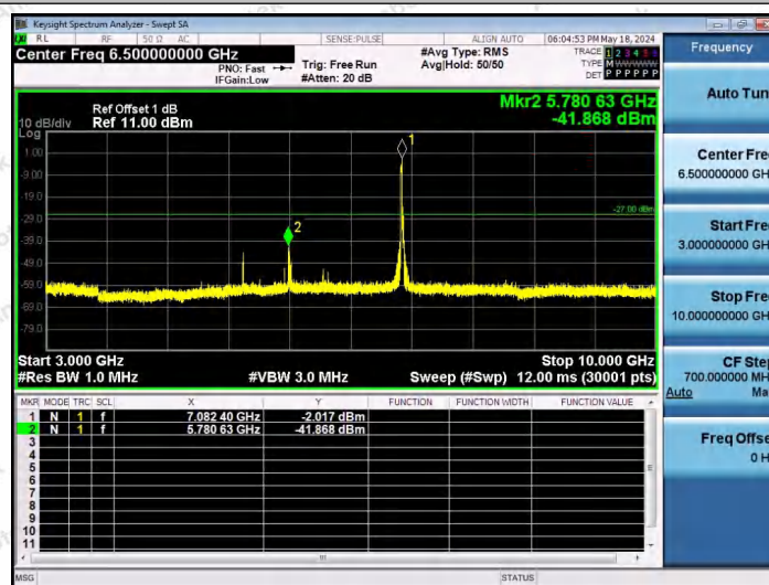
11AX40SISO-Ant1-7085-242Tone-RU61-3000~10000-PASS
