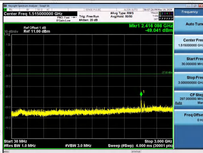
11AX40SISO-Ant1-7085-242Tone-RU62-30~3000-PASS
