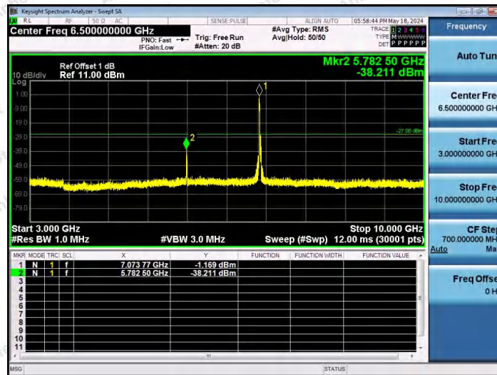
11AX40SISO-Ant1-7085-106Tone-RU53-3000~10000-PASS
