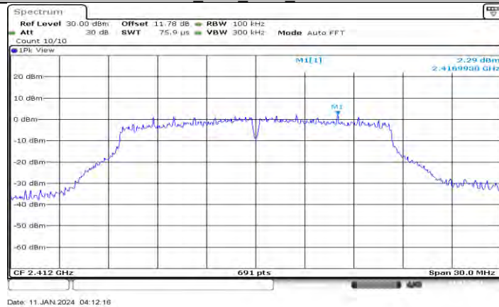
11G-CDD Ant1 2412_0~Reference
