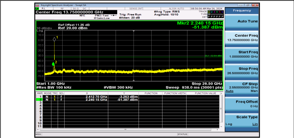
11G-Ant1-2412-1000~26500-PASS
