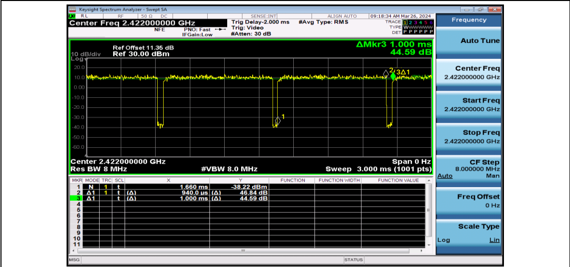
NTNV-11N40SISO-Ant1-2422
