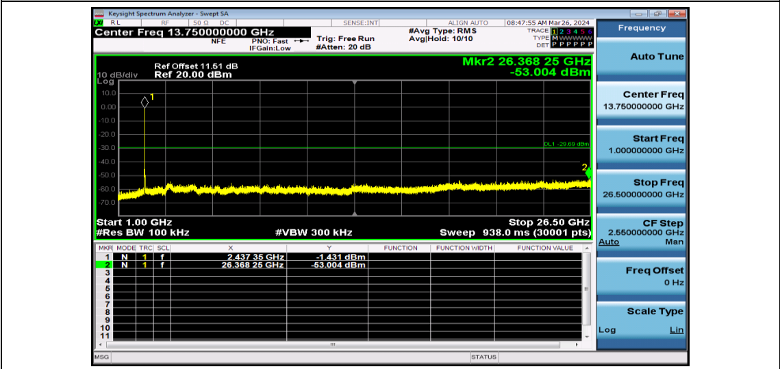
11B-Ant1-2437-1000~26500-PASS
