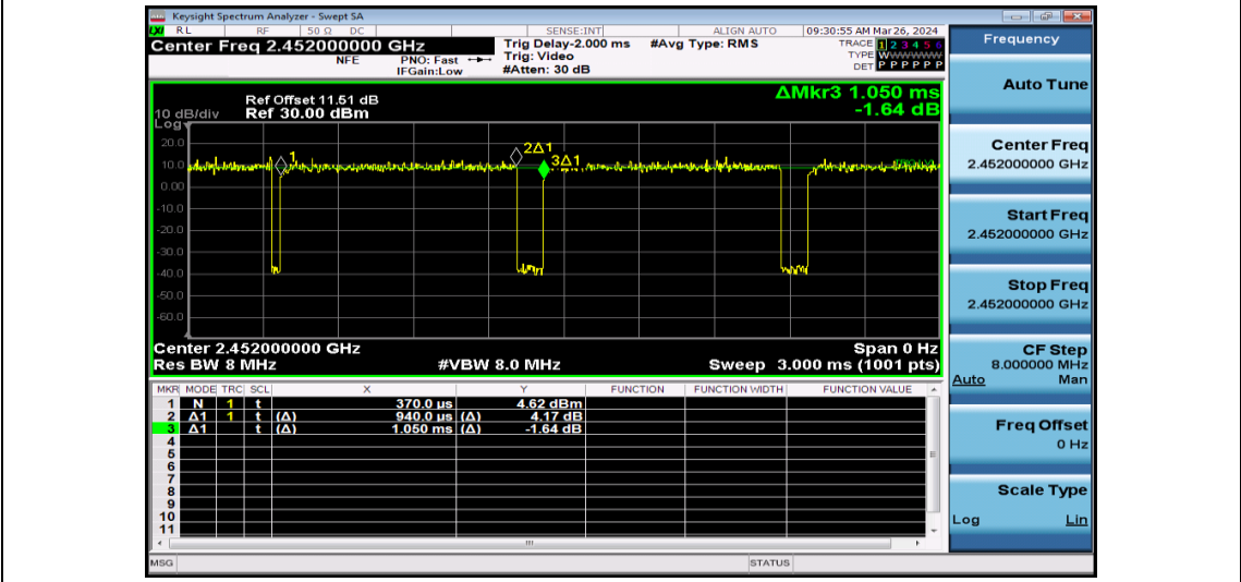
NTNV-11N40SISO-Ant1-2452
