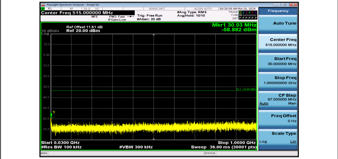
11N40SISO-Ant1-2437-30~1000-PASS
