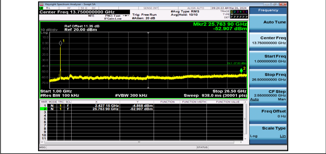
11N40SISO-Ant1-2422-1000~26500-PASS
