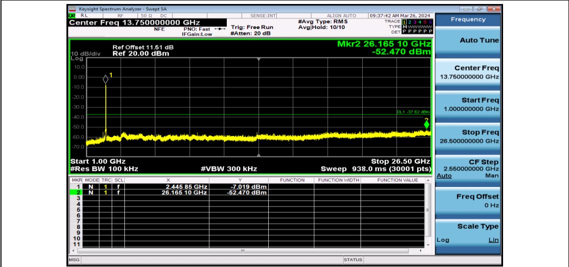
11N40SISO-Ant1-2452-1000~26500-PASS
