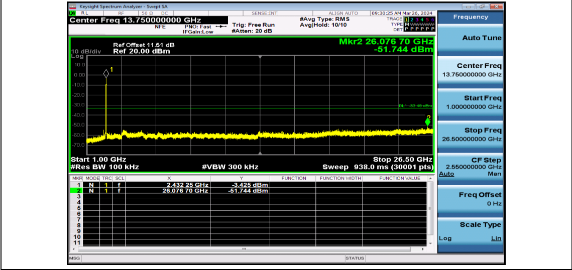
11N40SISO-Ant1-2437-1000~26500-PASS
