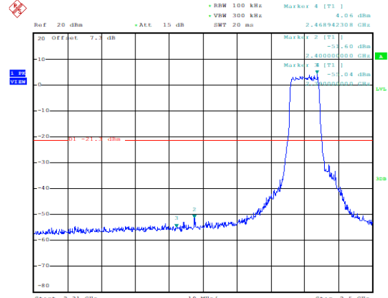
Band Edges (802.11g, Ch11)
