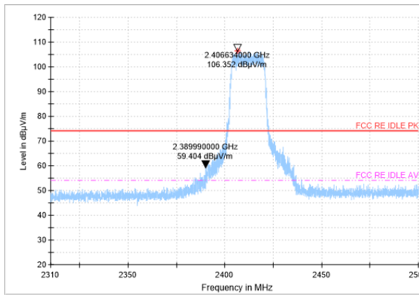
Peak detector
