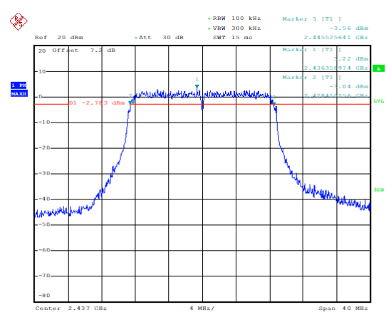
Occupied 6dB Bandwidth (MHz) (802.11n-20MHz, Ch6)
