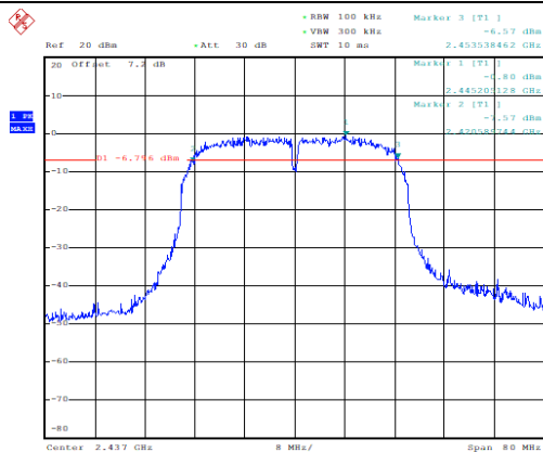
Occupied 6dB Bandwidth (MHz) (802.11n-40MHz, Ch6)
