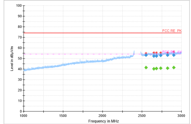
Radiated Spurious Emission (802.11n-20MHz, Ch11, 1GHz~3GHz)
