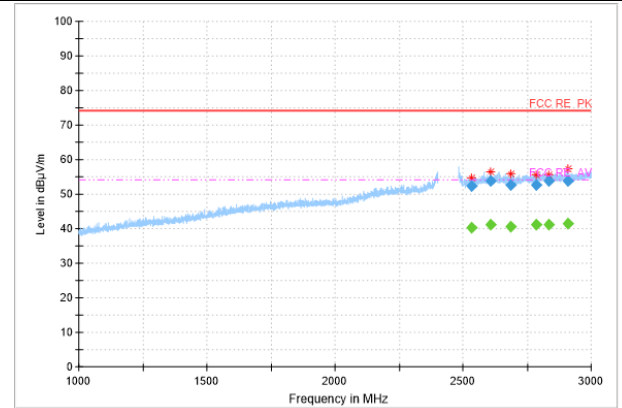
Radiated Spurious Emission (802.11g, Ch11, 1GHz~3GHz)
