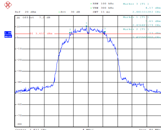
Occupied 6dB Bandwidth (MHz) (802.11b, Ch6)
