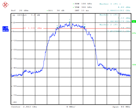
Occupied 6dB Bandwidth (MHz) (802.11b, Ch11)
