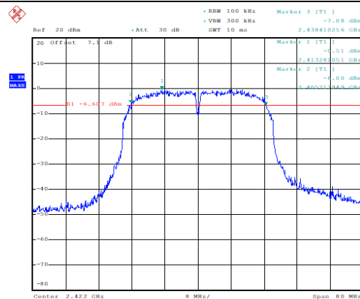
Occupied 6dB Bandwidth (MHz) (802.11n-40MHz, Ch3)
