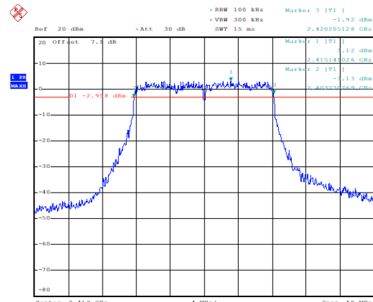
Occupied 6dB Bandwidth (MHz) (802.11g, Ch1)
