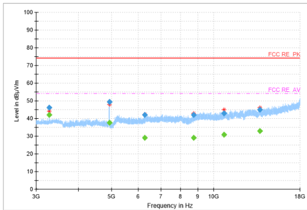
Radiated Spurious Emission (802.11g, Ch11, 3GHz~18GHz)
