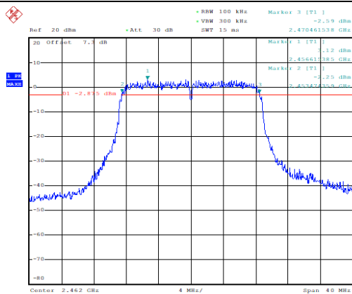
Occupied 6dB Bandwidth (MHz) (802.11n-20MHz, Ch11)
