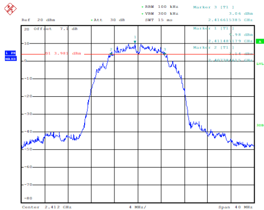
Occupied 6dB Bandwidth (MHz) (802.11b, Ch1)
