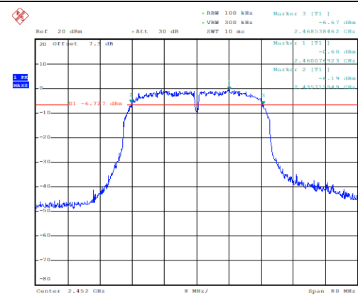
Occupied 6dB Bandwidth (MHz) (802.11n-40MHz, Ch9)
