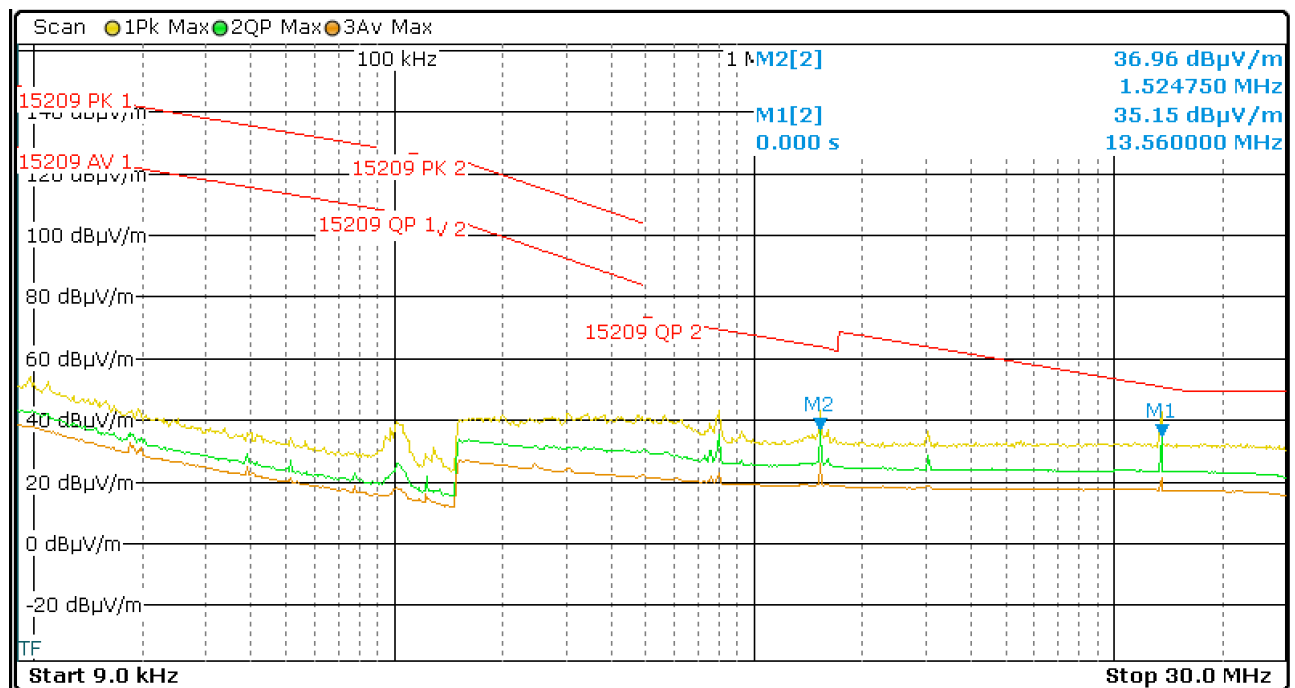
Figure 11: Chart of radiated emissions test below 30 MHz, EUT position Y, antenna polarization parallel, with tag
