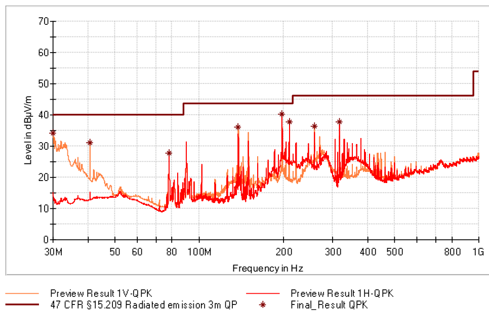
Figure 12: Chart of radiated emissions test from 30 MHz to 1 GHz, EUT position Y, antenna polarization horizontal and vertical, with tag
