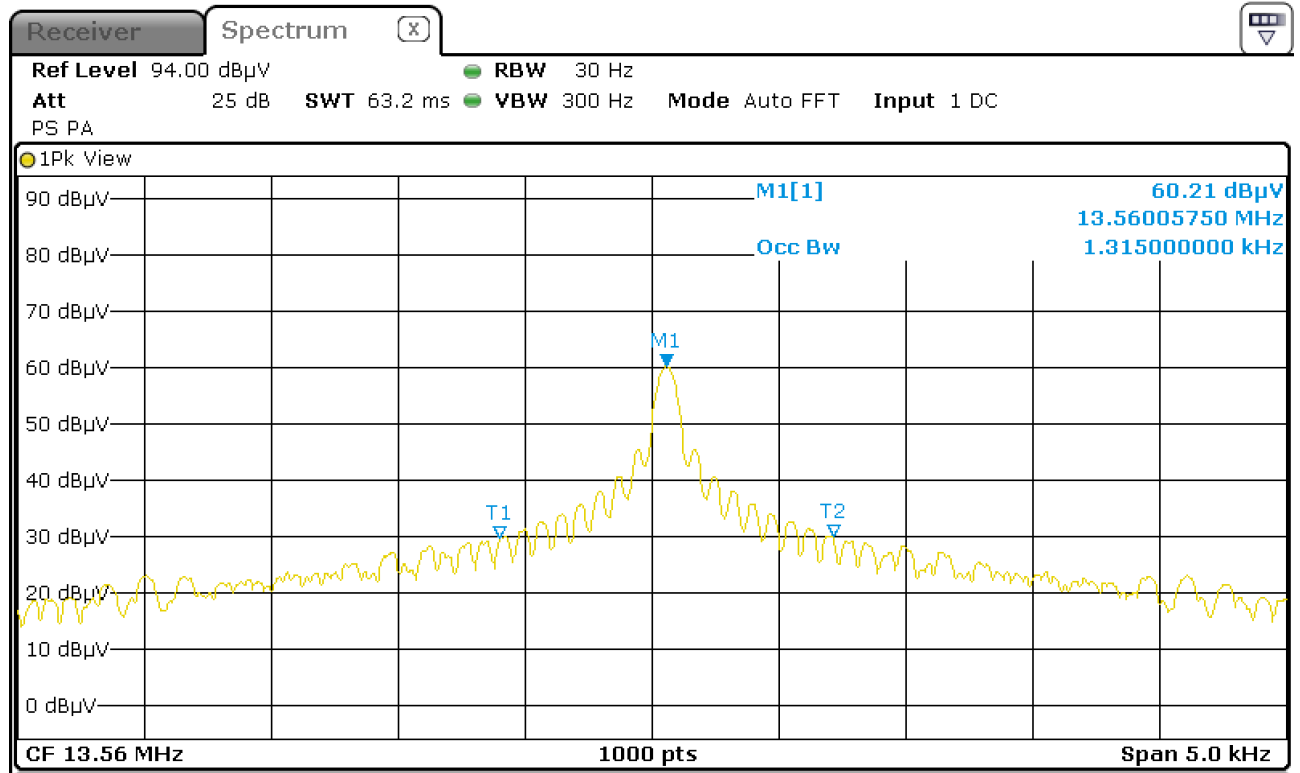
Figure 9: Chart of occupied bandwidth test, without tag
