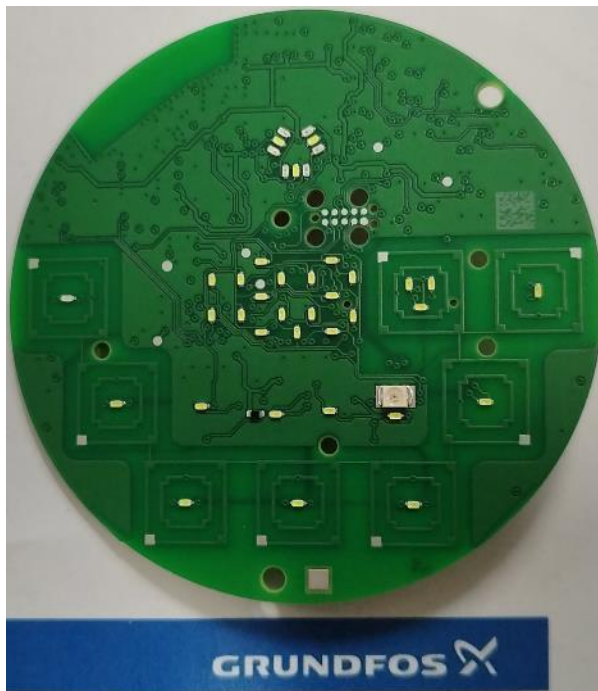
Figure 1 – Top side of 92710890 Module
