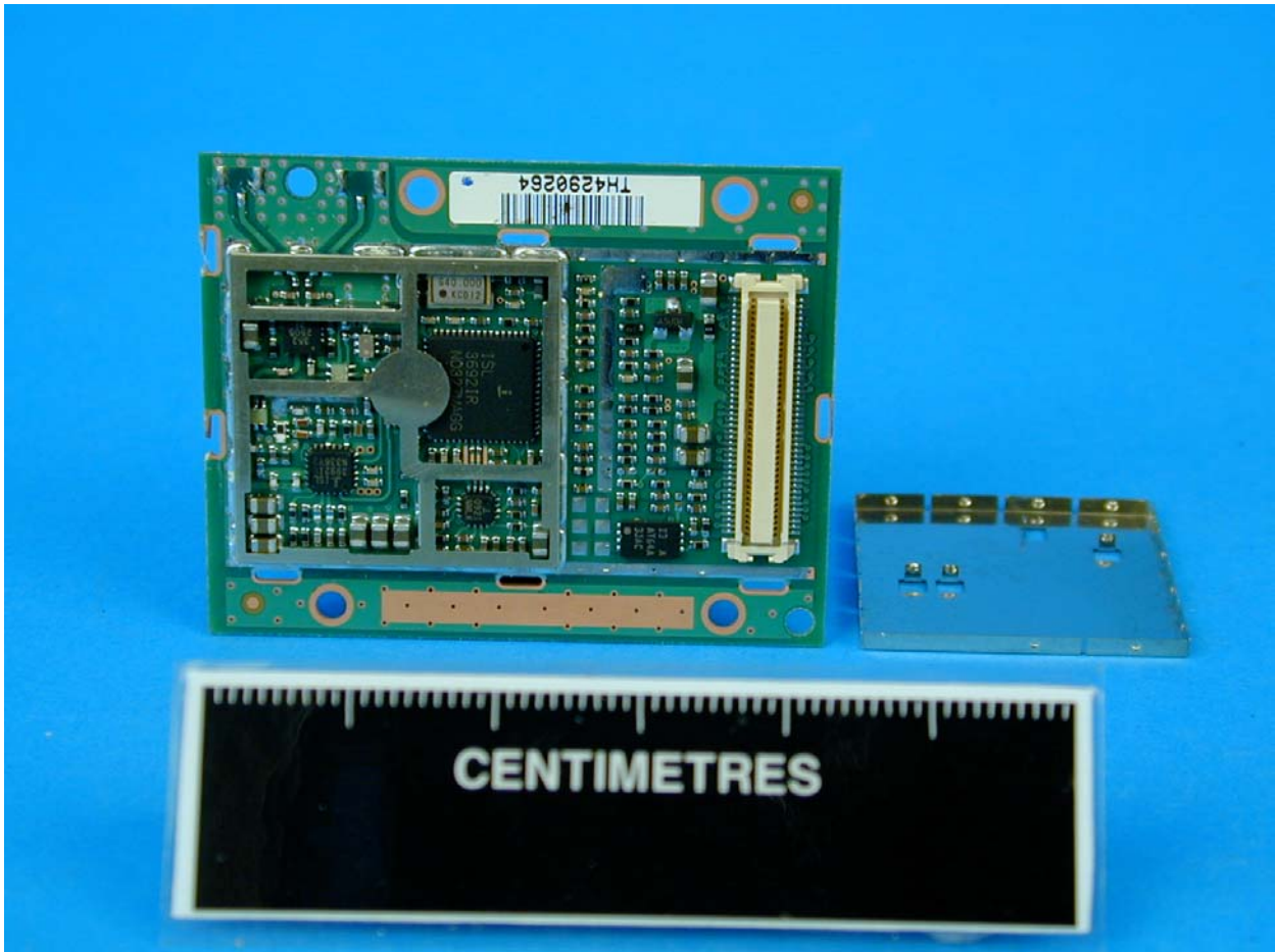
Internal View 2 21-21160-01
