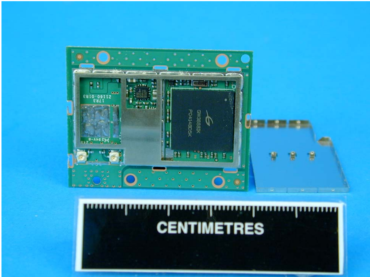
Internal View 1 21-21160-01
