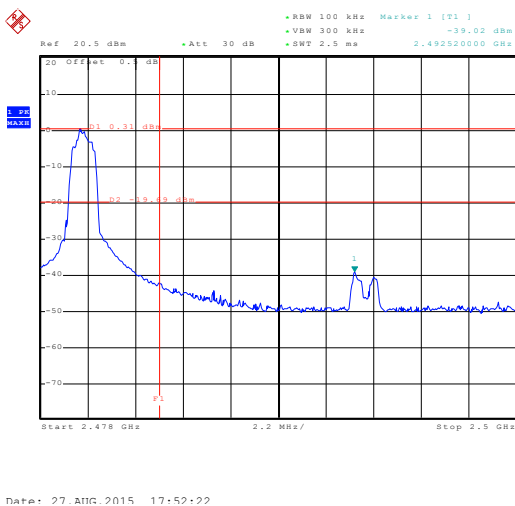
No-hopping mode
