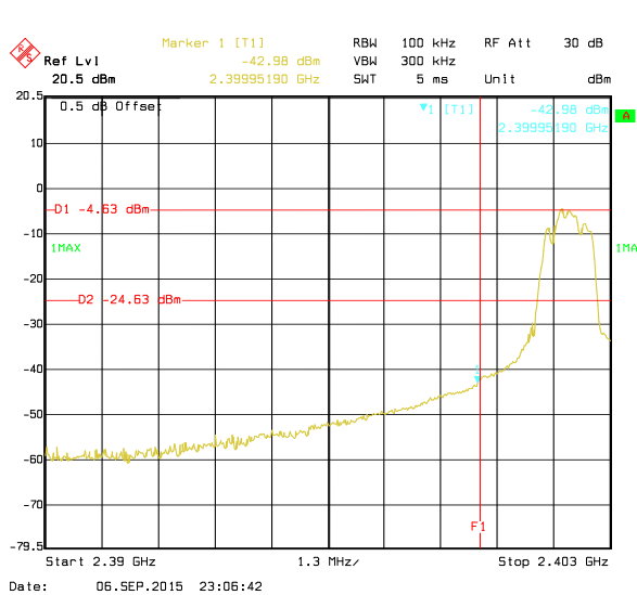
No-hopping mode
