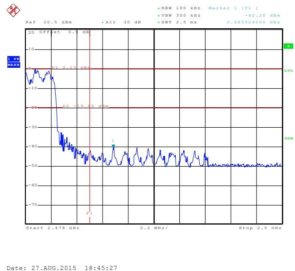
Hopping mode
