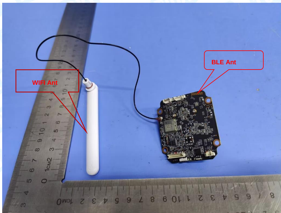
Photo 9 Antenna Appearance
