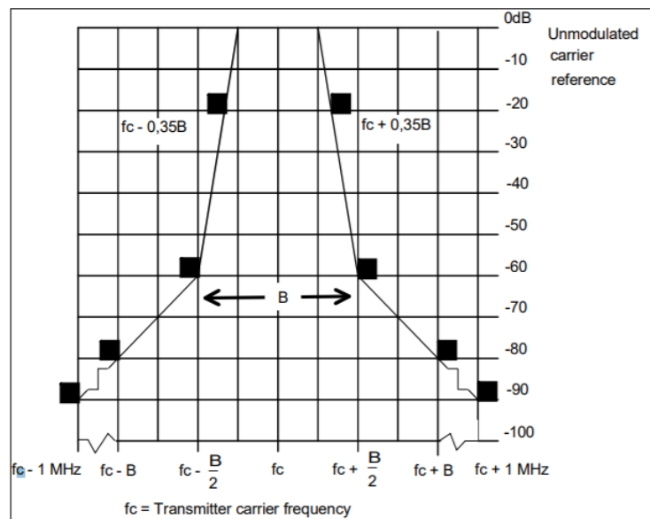
Figure 3: Spectrum mask for analogue systems in all bands - ETSI EN 300 422-1
