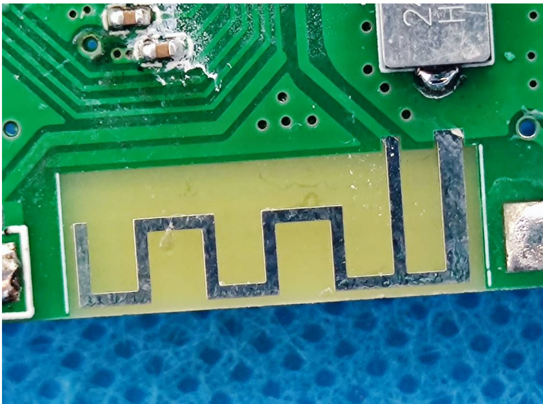
Bluetooth Antenna
