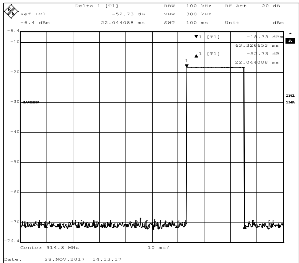
Figure 2 – Duty Cycle
