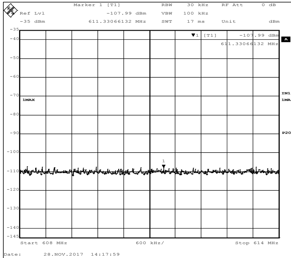
Figure 16 - Band-edge Measurement, Low Channel, Restricted Frequency, Hopping The plot shows an uncorrected measurement, used for relative measurements only.
