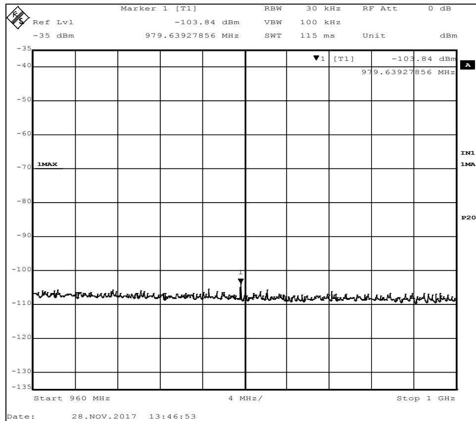
Figure 19 - Band-edge Measurement, High Channel, Restricted Frequency, Continuous Transmit
