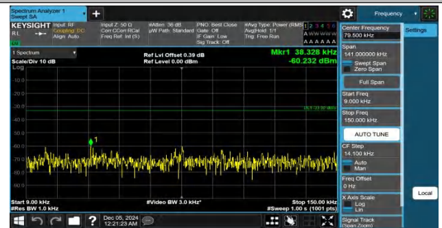
Band26(824-849)-1.4MHz-QPSK-26915-1RB#5-0.009~0.15-PASS
