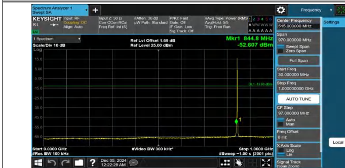
Band26(824-849)-1.4MHz-QPSK-27033-1RB#0-30~1000-PASS
