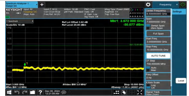
Band26(824-849)-1.4MHz-QPSK-26915-1RB#5-3000~10000-PASS S
