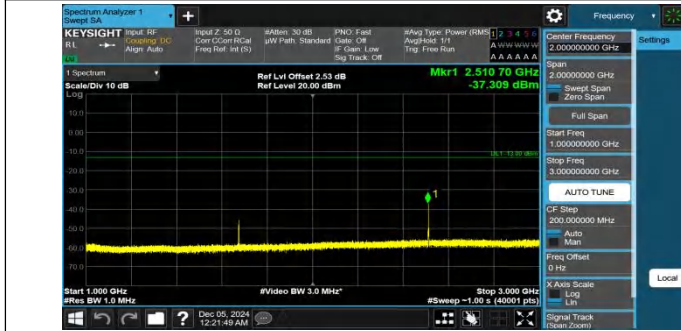
Band26(824-849)-1.4MHz-QPSK-26915-1RB#5-1000~3000-PASS
