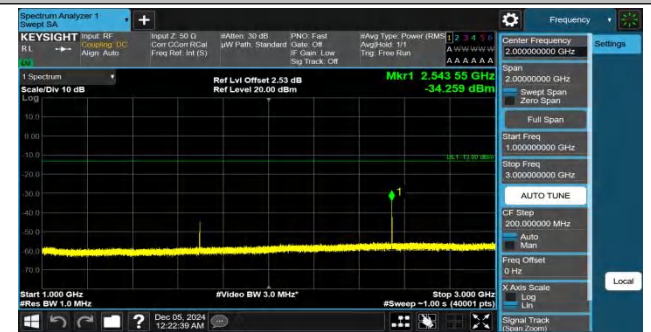
Band26(824-849)-1.4MHz-QPSK-27033-1RB#0-1000~3000-PASS
