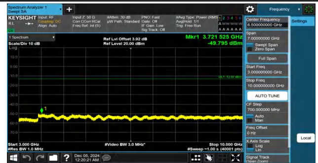
Band26(824-849)-1.4MHz-QPSK-26797-1RB#5-3000~10000-PASS
