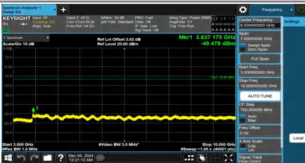
Band26(824-849)-1.4MHz-QPSK-26915-1RB#0-3000~10000-PASS
