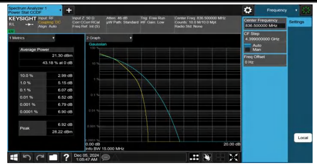
Band26(824-849)-15MHz-16QAM-26915-75RB#0-PASS
