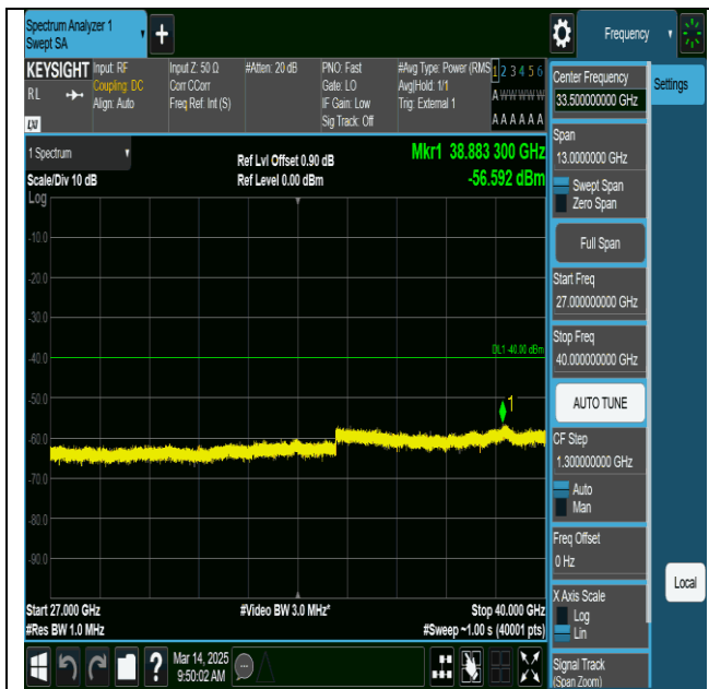
48-48-20MHz-20MHz-QPSK-QPSK-55340-55538-1RB#0-ORB#0-27000~40000MHz-PASS
