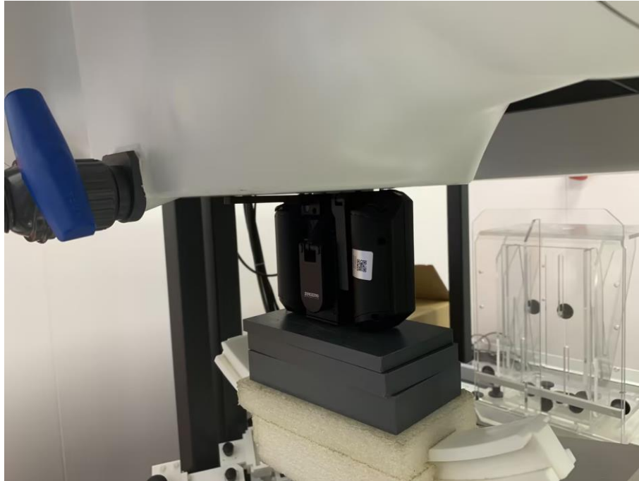
Body Top1
