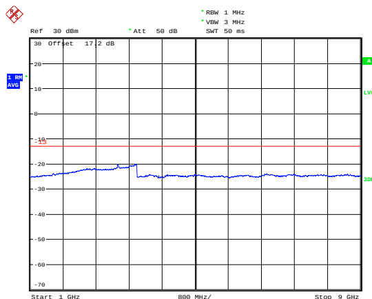
LTE Band 5 1.4MHz CH-Low 1GHz ~9GHz
