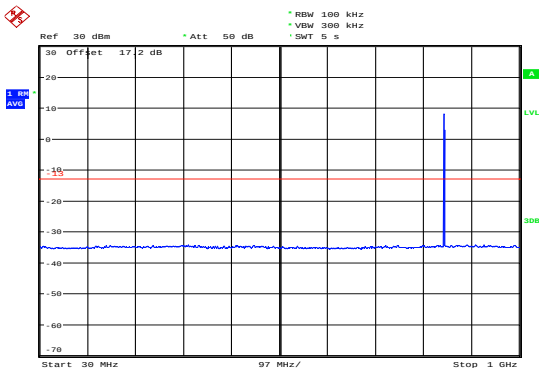
LTE Band 5 1.4MHz CH-High 30MHz~1GHz
