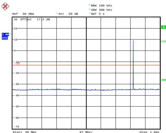
LTE Band 5 1.4MHz CH-Low 30MHz~1GHz
