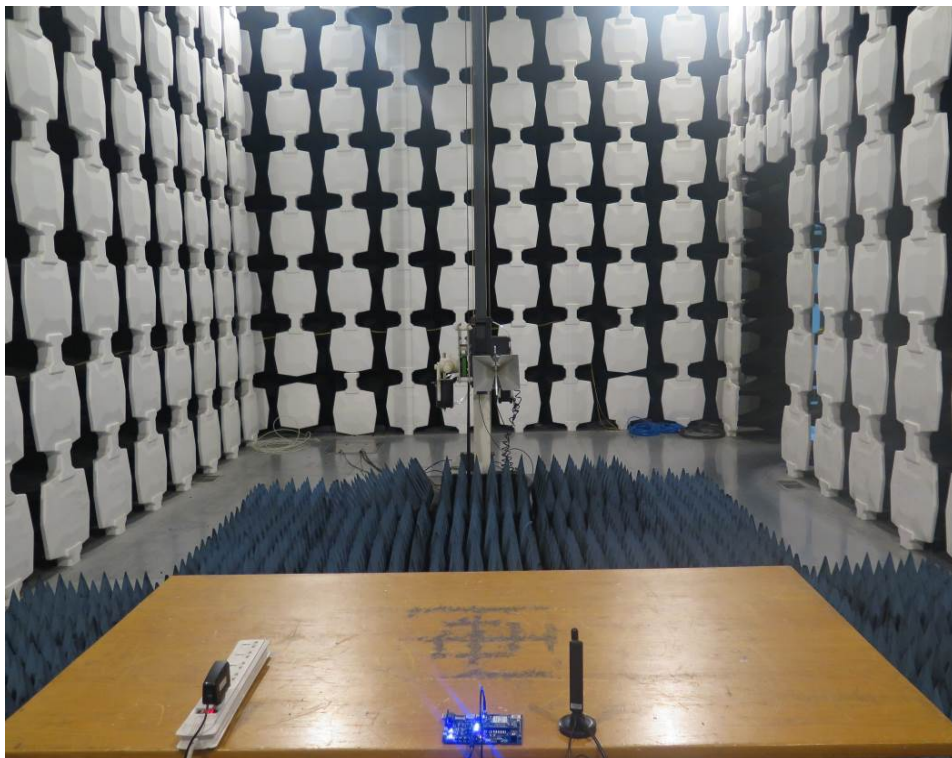
Pic2. Radiated emissions(1G-18G)
