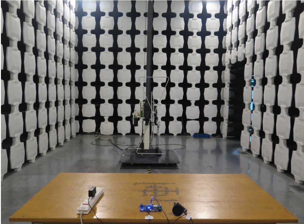
Pic1. Radiated emissions(30M-1G)
