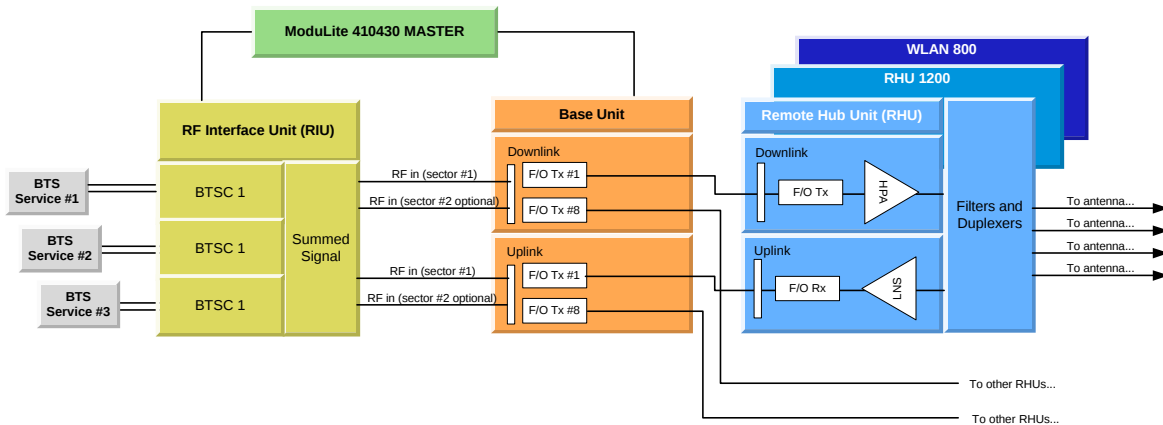
Figure 1-1. MobileAccess™ System Block Diagram
