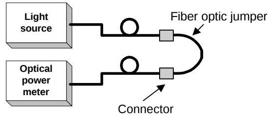
Figure 4-5: Single Point Test
