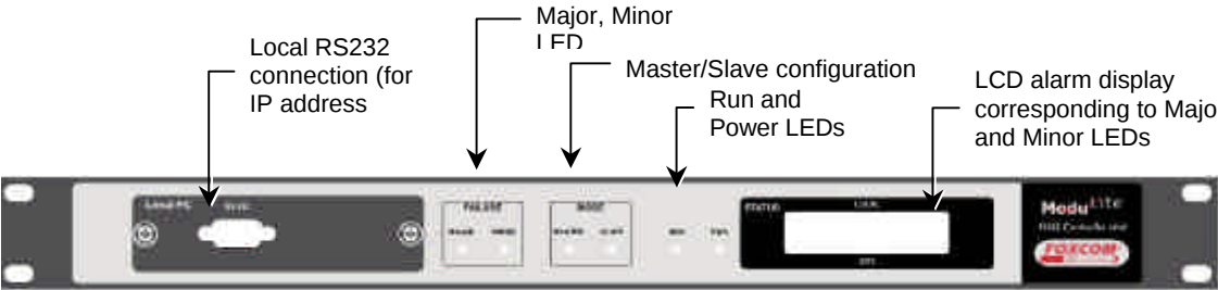
Figure 2-8. MobileAccess 410 Front Panel
