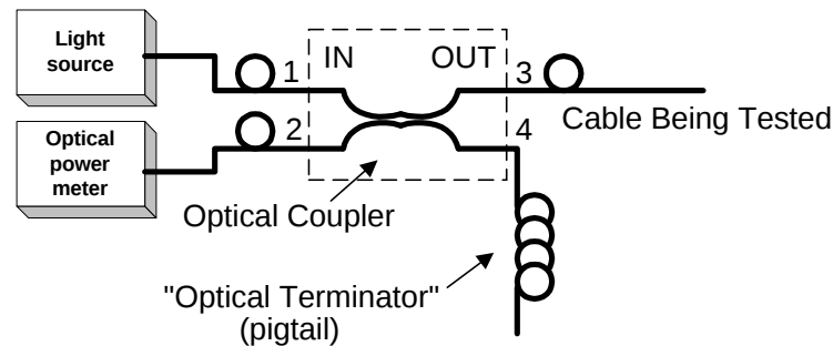
Figure 4-6: Optical Return Loss Measurement
