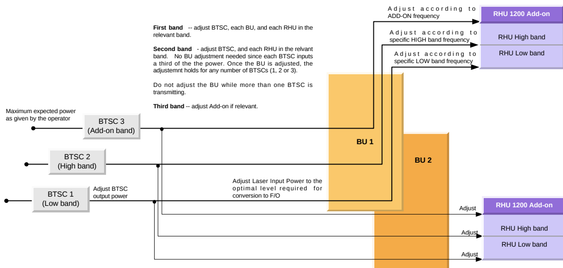
Figure 4-1. Main or Independent Building with RIU
