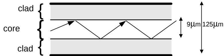
Figure 4-2: Fiber Optic Cable Structure
