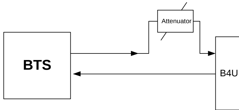
Figure 3-6: Example: Two port BTS/RBS connected to B4U.
