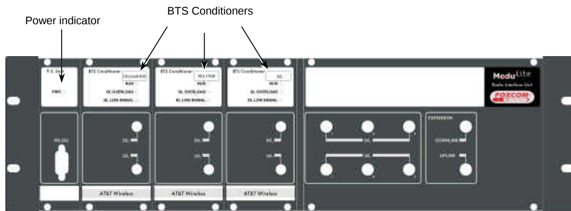
Figure 2-1. RIU Front Panel
