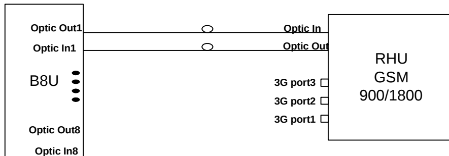
Figure 3-11:UMTS Ready -System Configuration
