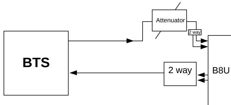
Figure 3-7: Example: Two port BTS/RBS connected to B8U with six optic links
