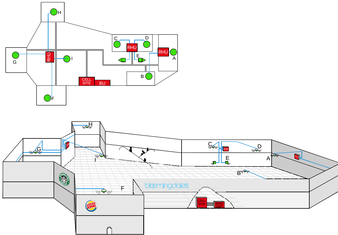
Figure 3-1: Horizontal Layout Installation
