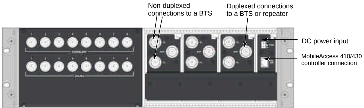
Figure 3-8. RIU Rear Panel showing the RF Connection
