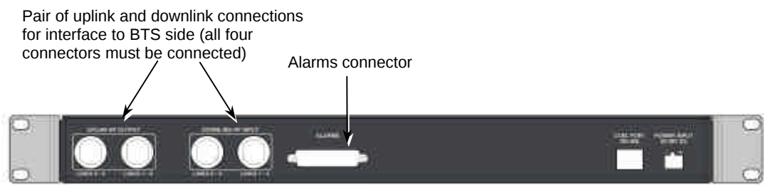
Figure 2-5. Base Hub Unit Rear Panel (RF Connections)
