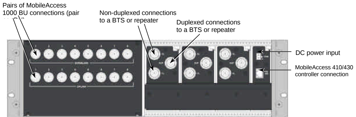
Figure 2-2. RIU Rear Panel showing the RF Connection
