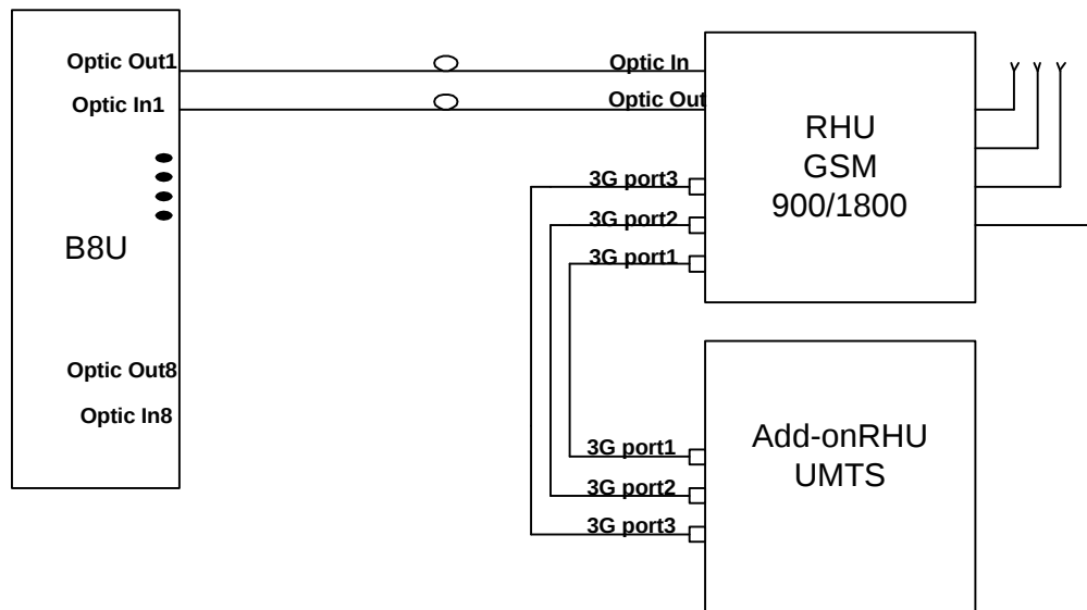
Figure 3-12: Example - MobileAccess™ UMTS Ready Full Installation
