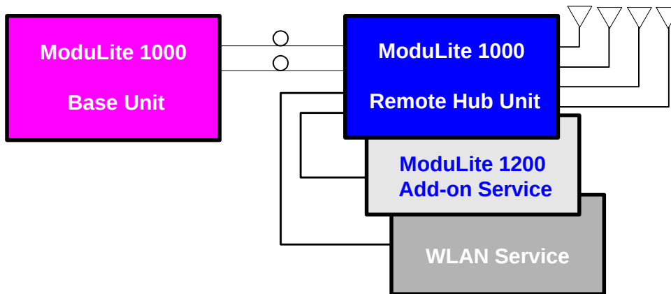
Figure 5: MobileAccess 1000/1200 BU – RHU Plus Add-on Plus WLAN Configuration
