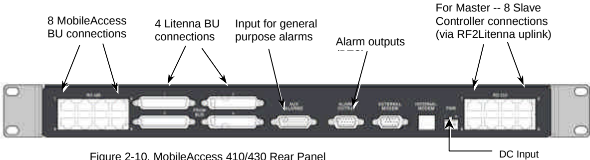
Figure 2-10. MobileAccess 410/430 Rear Panel
