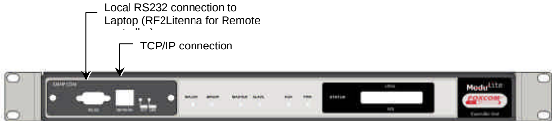
Figure 2-9. MobileAccess 430 Front Panel
