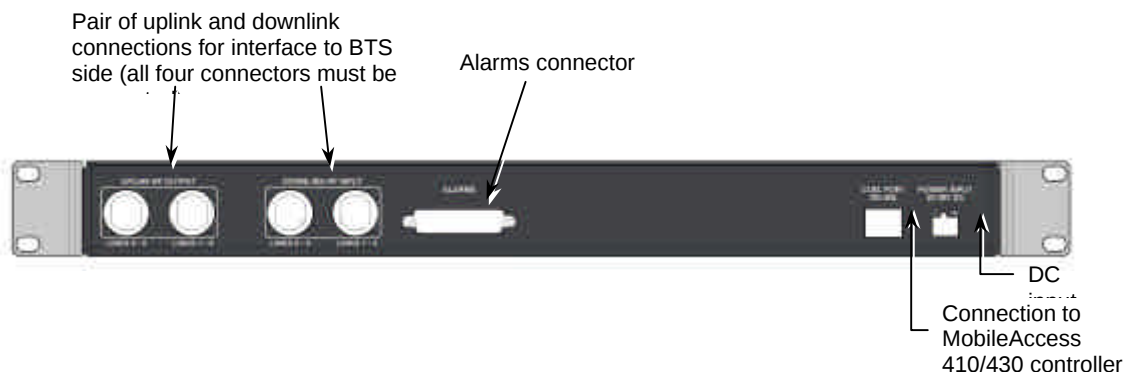
Figure 3-3. Base Hub Unit Rear Panel (RF Connections)
